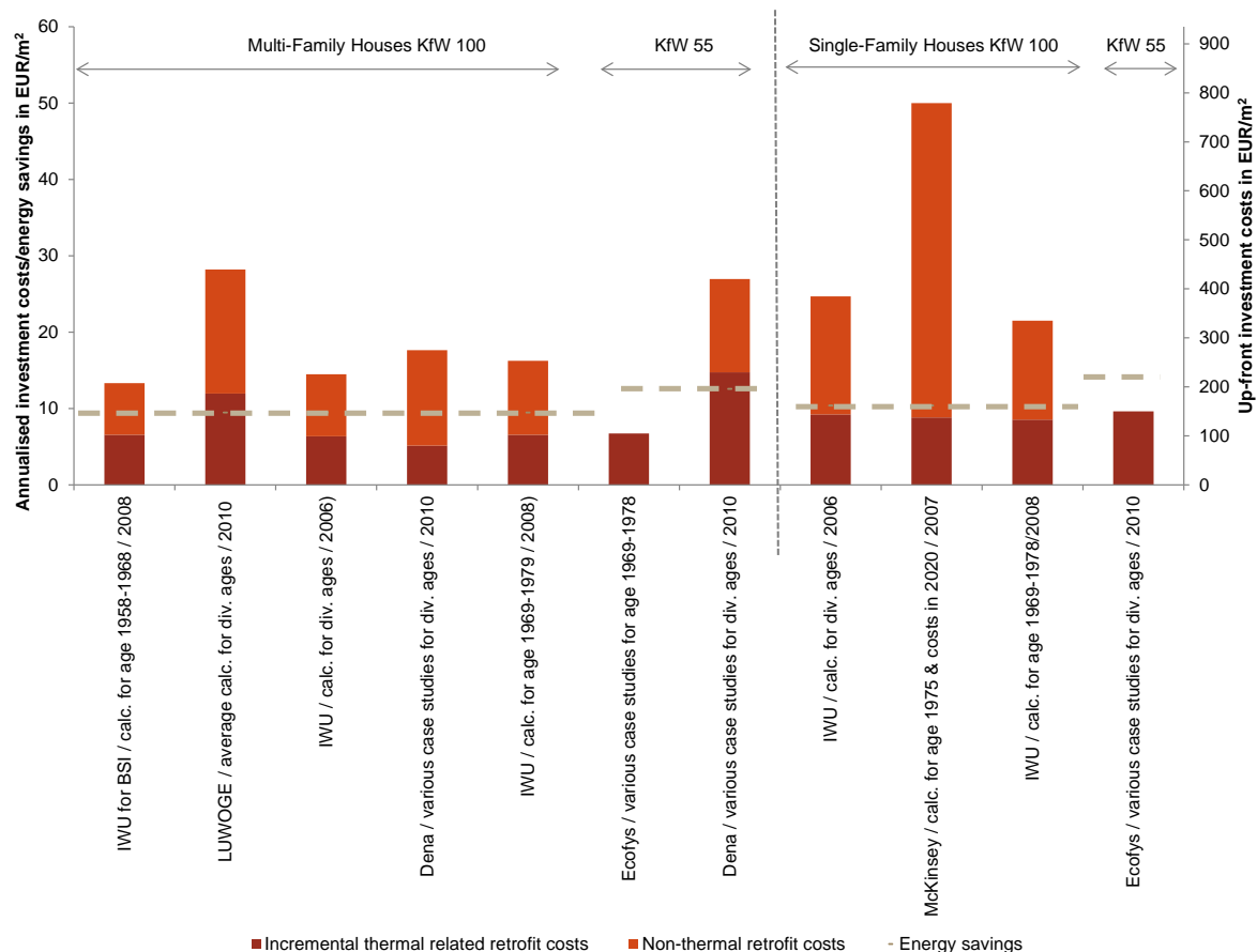
Figure 2: Summary of several retrofit costs studies. The figure depicts thermal and other (non-thermal) retrofit costs versus saved energy costs [1]. The left axis of the graph shows the annualized costs and savings, while the right axis of the graph shows costs as up front investments.
