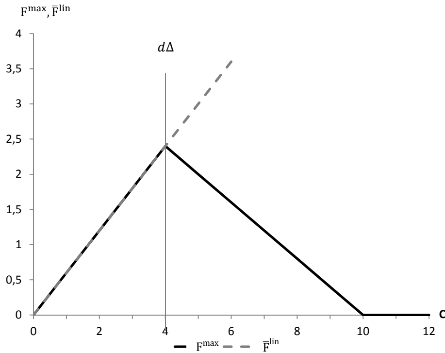
Figure 7: Comparison of the maximal fee \bar{F}^{max} and the linear fee \bar{F}^{lin} for an ATR depending on the pre-audit net cashflow C
