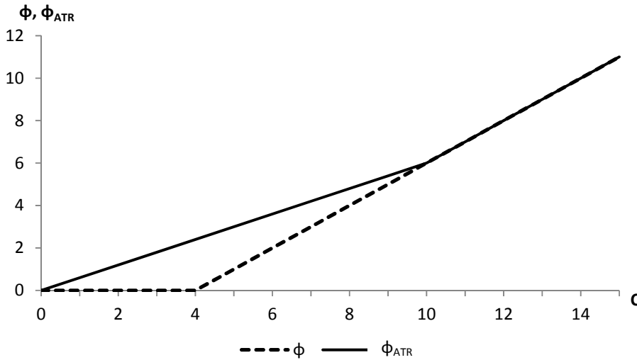
Figure 2: Objective functions with ( \phi_{ATR} ) and without an ATR ( \phi ) depending on the pre-audit net cashflow C
