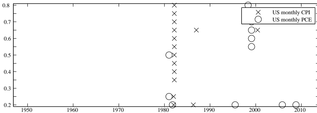
Figure 12: Estimated break points at different quantiles (monthly, standardized). Notes: The graph shows breakpoints estimated with the SQ_{\tau} -test at all quantiles \tau \in \{0.20, 0.25, \dots, 0.80\} (vertical axis) after controlling for mean and volatility shifts for US CPI and PCE inflation on the 5% significance level.
