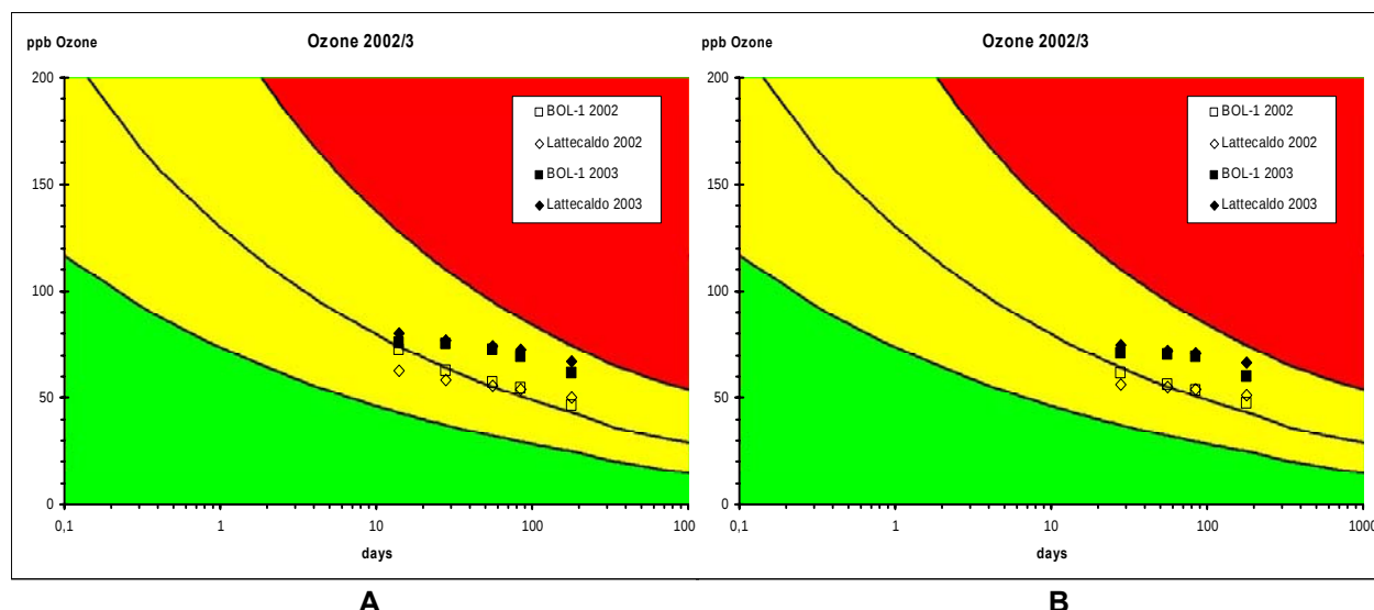
Figure 3.5.3-10: Hourly mean ozone concentration aggregated to 14 and 28 day means for the vegetation period of the years 2002 and 2003 (April-September) for the 2 stations Lattecaldo (CH) and Boll (Italy) to simulate measurements with passive samplers over the recommended 14-day exposure period (A) and 28-day period (B).
