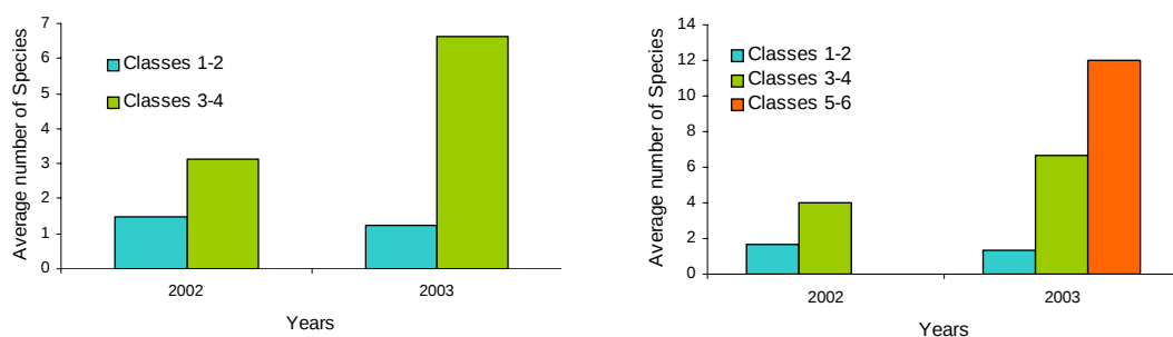
Figure 3.5.3-8: Average number of symptomatic species per plot in common plots to 2002 and 2003 where ozone measurements were carried out (countries: Italy, Spain, and Switzerland). The left graph is based in the average April-September classes reached in these plots, whereas the in the right graph calculations are based in the maximum 2-week values measured in this period.
