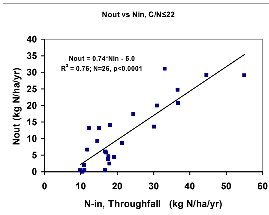
Figure 3.4.3-2: N leaching fluxes ( \text{kg N ha}^{-1} \text{ y}^{-1} ) against N input in throughfall for IFEF forests with C:N \leq 22
