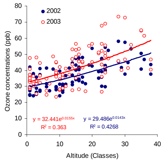
Figure 3.5.3-4: Regression analysis for ozone concentrations (ppb) of Level II plots versus latitude (a) and (b) altitude respectively for the years 2002 and 2003.
