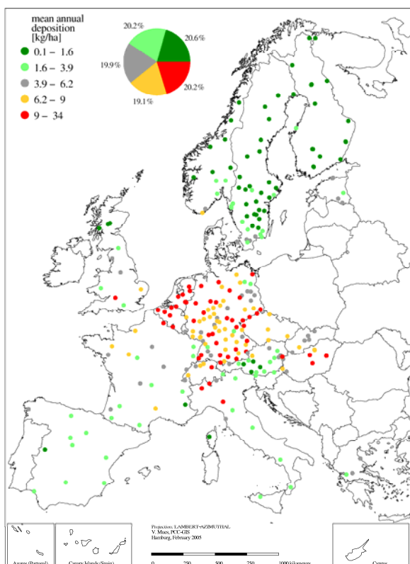
Figure 3.2.3.1-6: Mean annual ammonium ( \text{N-NH}_4 ) throughfall deposition 1999 to 2001.
