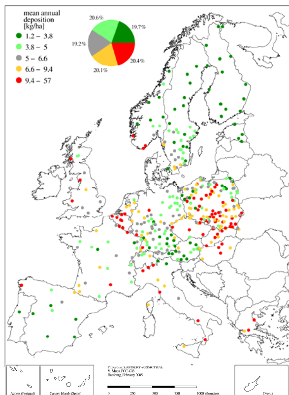
Figure 3.2.3.1-2: Mean annual sulphate (S-SO 4 ) bulk deposition 1999 to 2001.
