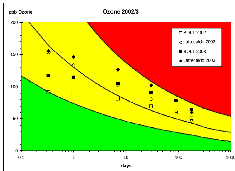
Figure 3.5.3-9: (A) AOT40 (ppb.h) for years 2002 and 2003 at Lattecaldo (CH) and BOL1 (IT). White columns represent the AOT40 measured at 2 m and the grey columns represent the value corrected for canopy height assumed to be 1.1 as default value. The dotted horizontal lines represent the critical levels for 6 months. (B) Maximum permissible ozone concentrations (MPOC) for the same stations and years, calculated for the time intervals of 8 hrs and 1, 7, 30 and 90 days as well as a season mean (April-September).
