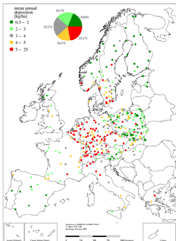
Figure 3.2.3.1-4: Mean annual nitrate (N-NO 3 ) bulk deposition 1999 to 2001.
