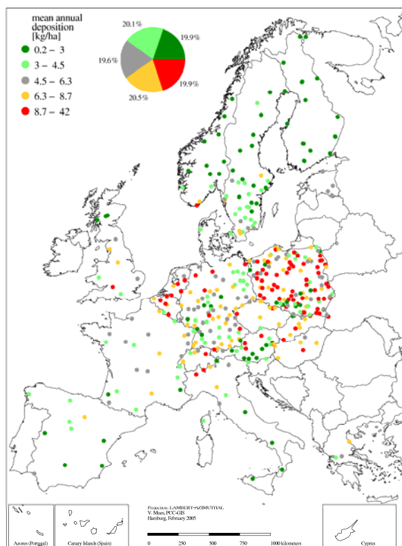
Figure 3.2.3.1-5: Mean annual ammonium ( \text{N-NH}_4 ) bulk deposition 1999 to 2001.
