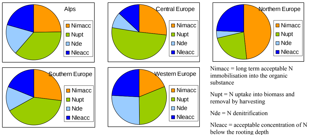
Figure 3.3.3.2-3: Composition of different sinks according to the SMB model in different regions.
