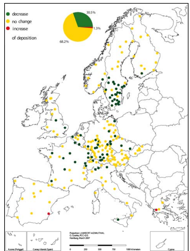
Figure 3.2.2.2-3: Trends in sulphur (S-SO 4 2- ) in throughfall deposition from 1999 to 2004.
