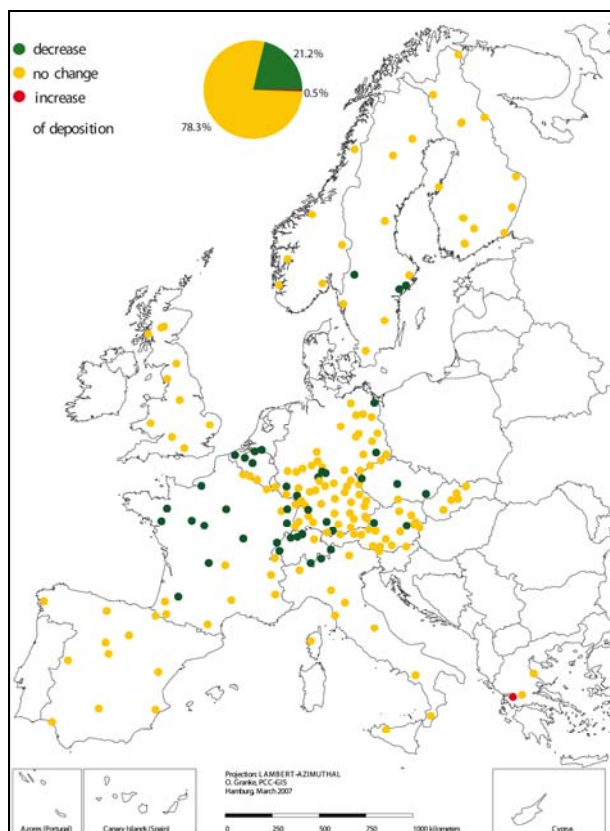
Figure 3.2.2.2-2: Trends in sulphur (S-SO 4 2- ) in bulk deposition from 1999 to 2004.
