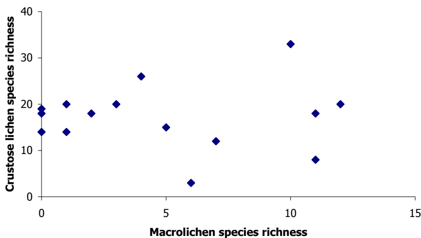
Figure 3.4.3-3: Relationship between macrolichen species richness and crustose lichen species richness ( p > 0.05 , n = 15 ).
