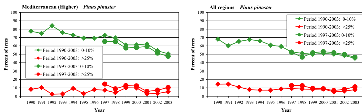
Figure 2.2.2.7-1: Shares of trees of defoliation 0-10% and >25% in two periods (1990-2003 and 1997-2003).
