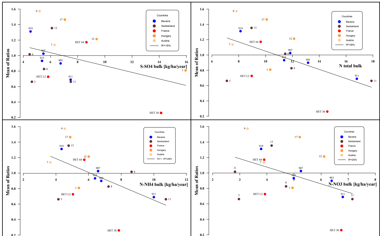
Figure 3.3.2.3-2a: Ratios between observed and modelled basal area increment (means by plot) of beech over deposition loads.
