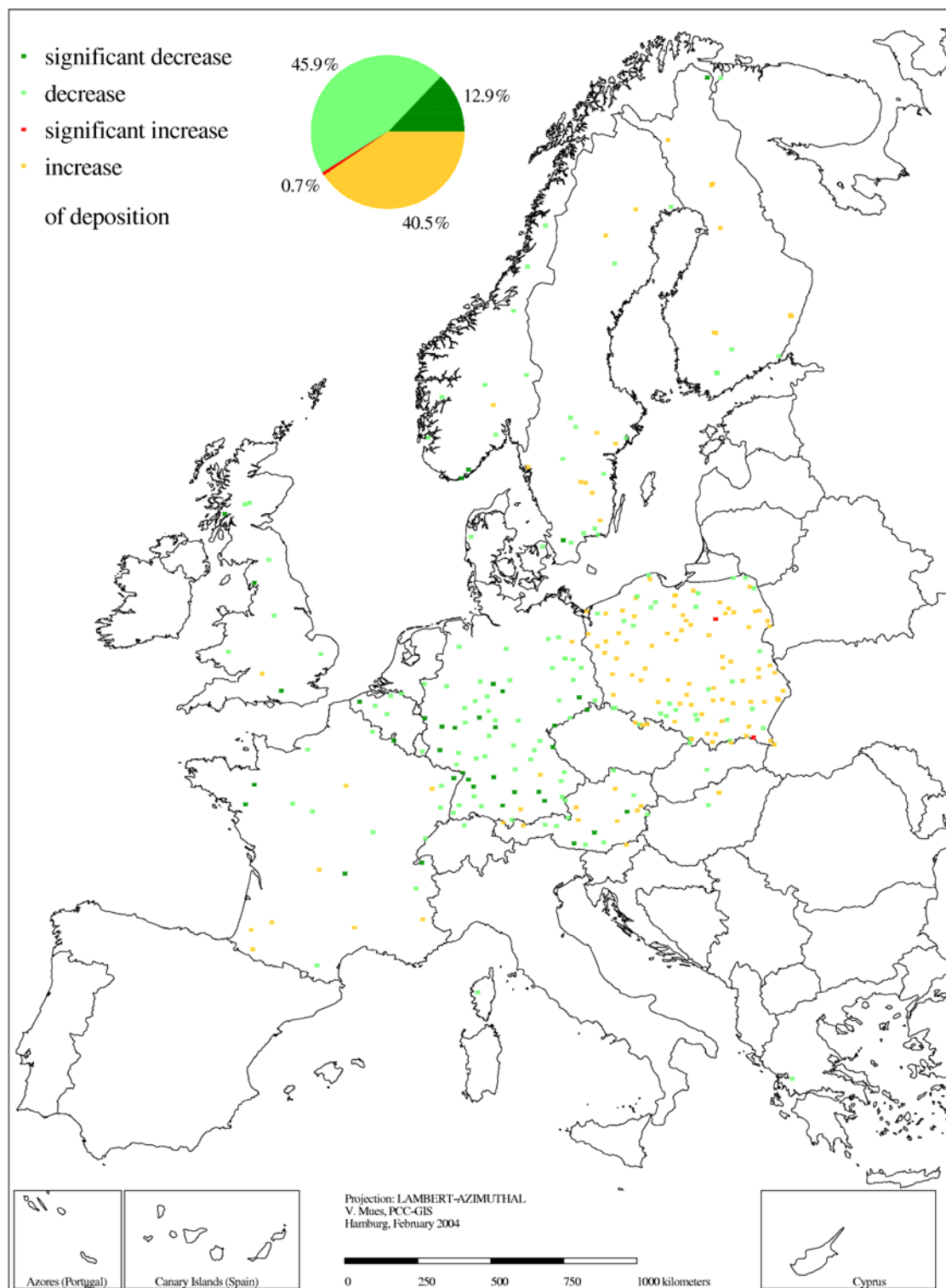
Figure 3.2.3.2-2: Linear trends of the volume weighted mean \text{N-NH}_4 concentration in \text{mg/l} between 1996 and 2001 at 294 Level II plots.
