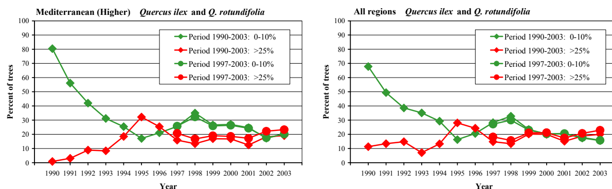
Figure 2.2.2.6-1: Shares of trees of defoliation 0-10% and >25% in two periods (1990-2003 and 1997-2003).
