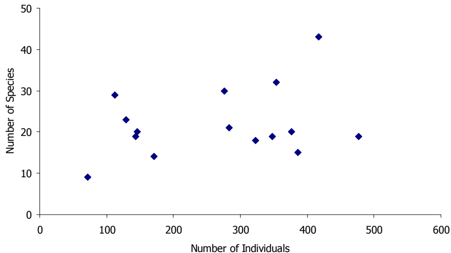
Figure 3.4.3-1: Relationship between the number of species and the number of individuals ( p > 0.05 , n = 15 ).
