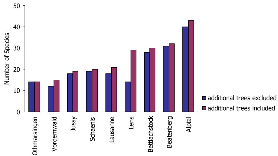
Figure 3.4.3-4: Lichen species richness with and without additional trees per plot.
