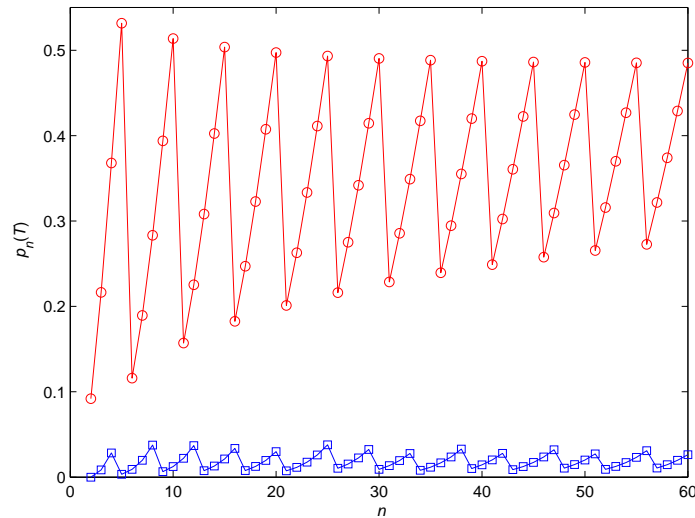
Figure 1 Probability of Excessive Delay for s_n = \lceil (1/5)n \rceil (above) and \tilde{s}_n^* = \lceil (1/5)n + 0.3\sqrt{n} + 1/2 \rceil (below), for r = 1/4 and T = 1/\mu
