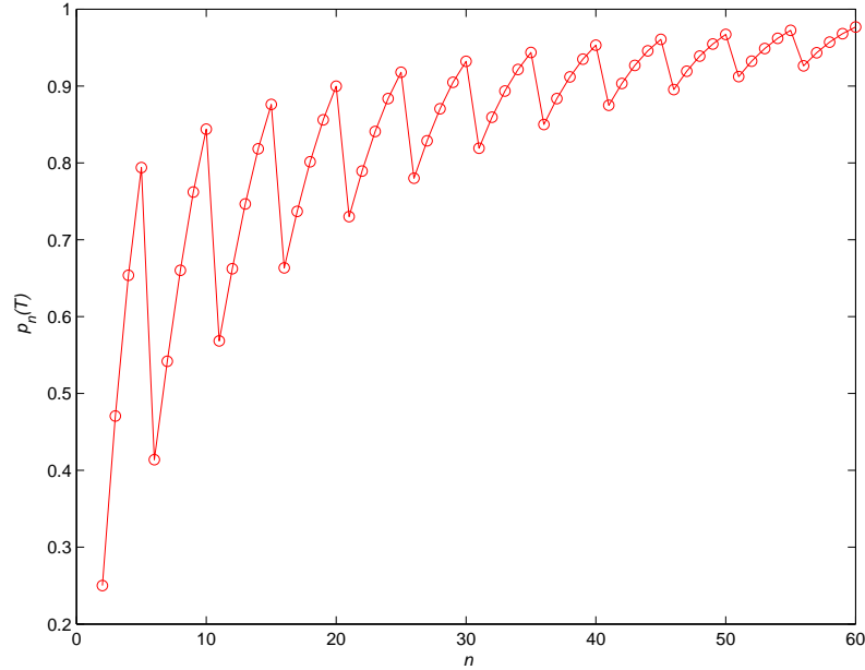
Figure 3 Probability of Excessive Delay for s_n = \lceil (1/5)n \rceil , r = 1/4 , T = 0
