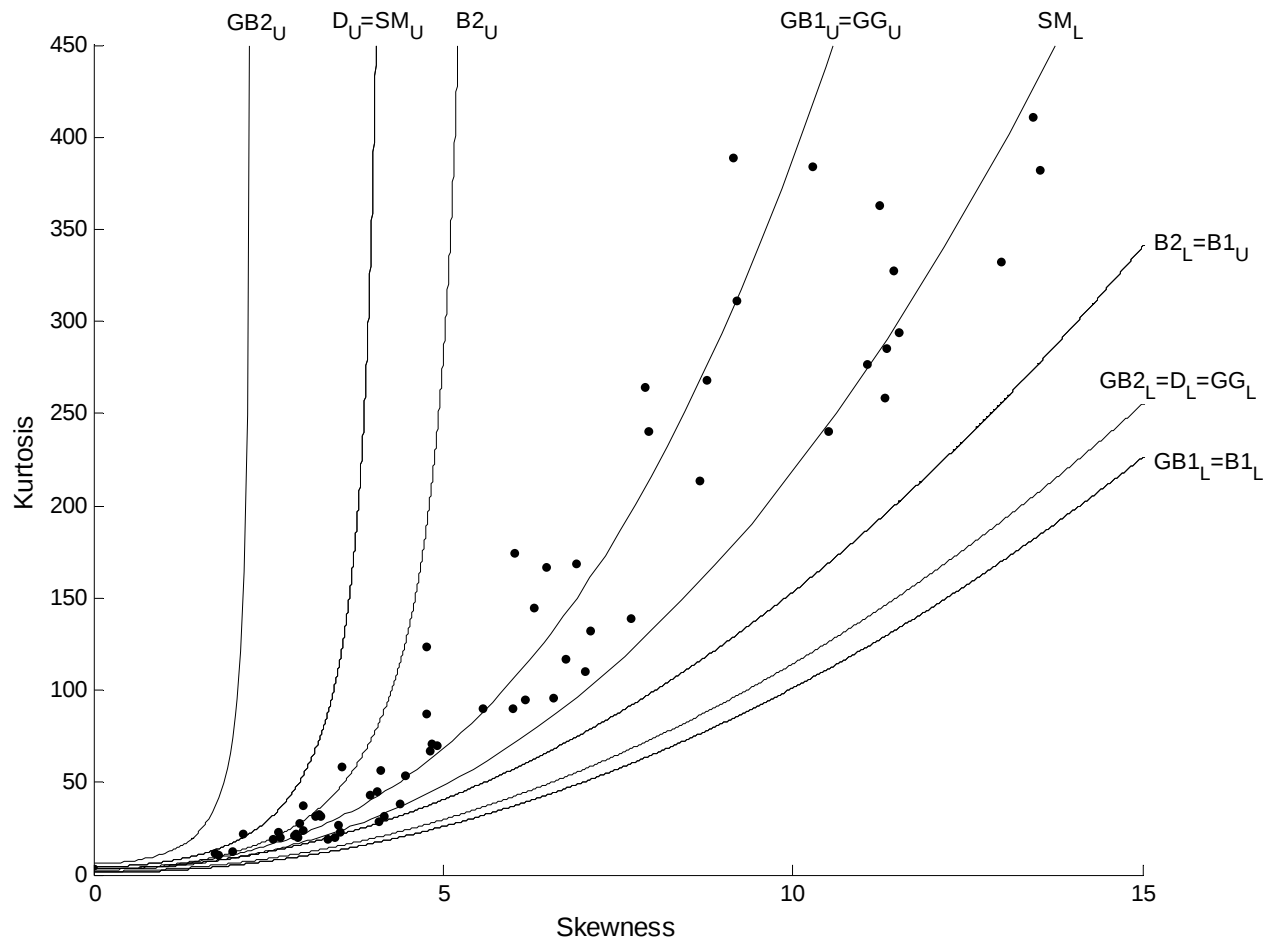
Figure 3. Skewness-kurtosis data points and skewness-kurtosis spaces
