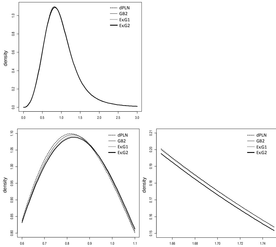
Fig. 4-1 Fitted PIDMs to equivalized gross income in Sweden, 2005
