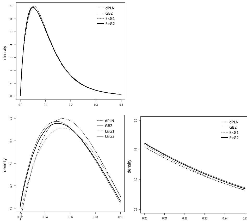
Fig. 4-2 Fitted PIDMs to non-equivalized gross income in Canada, 2004
