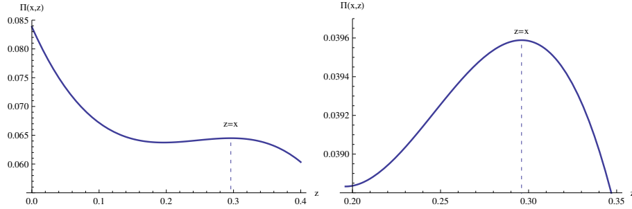
Figure 1: Left: Stationary point at z = x is not a global maximum for r = 0 ; Right: Stationary point at z = x is a global maximum for r \geq r_{\min}
