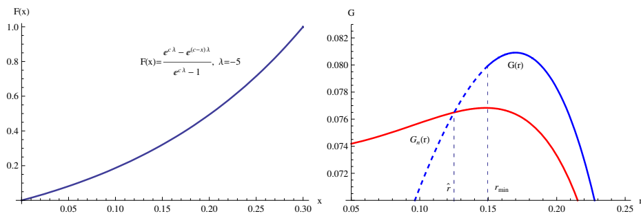
Figure 3: Truncated exponential distribution with a concentration on high cost reductions: cdf (left) and associated expected revenue of the innovator (right)
