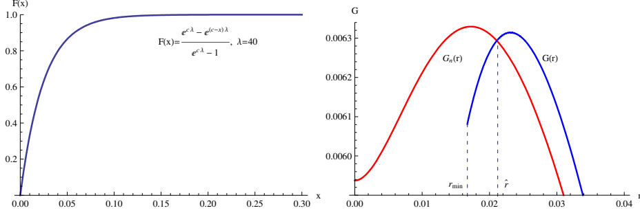
Figure 4: Truncated exponential distribution with a concentration on low cost reductions: cdf (left) and associated expected revenue of the innovator (right)
