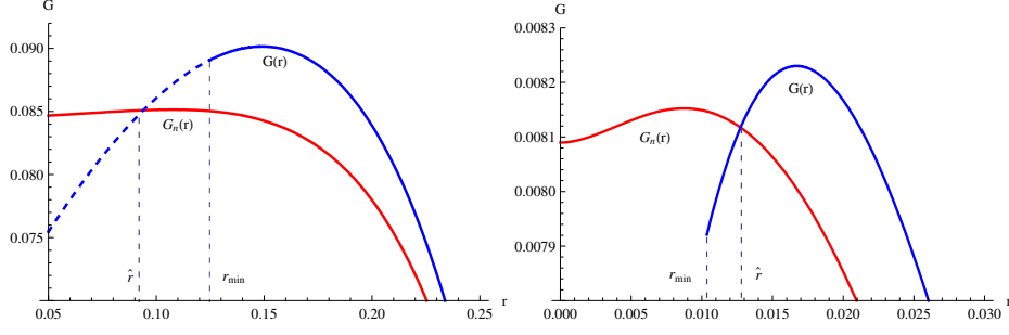
Figure 5: Expected revenue for truncated exponential distributions with a concentration on high cost reductions (left) and on low cost reductions (right)
