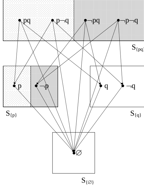
Figure 1: Event Structure
