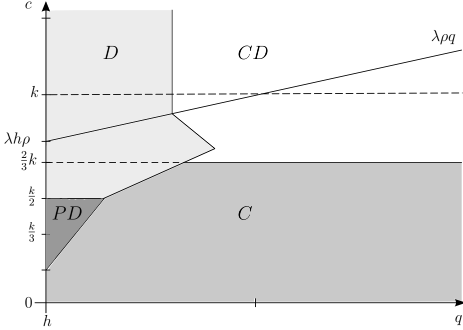
Figure 2: Optimal organizational structure for h < q
