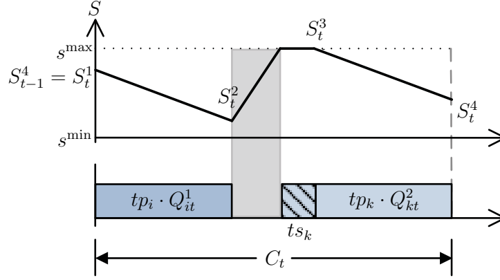
Figure 5: State variables for case \alpha = 0, \beta = 0, \gamma = 1
