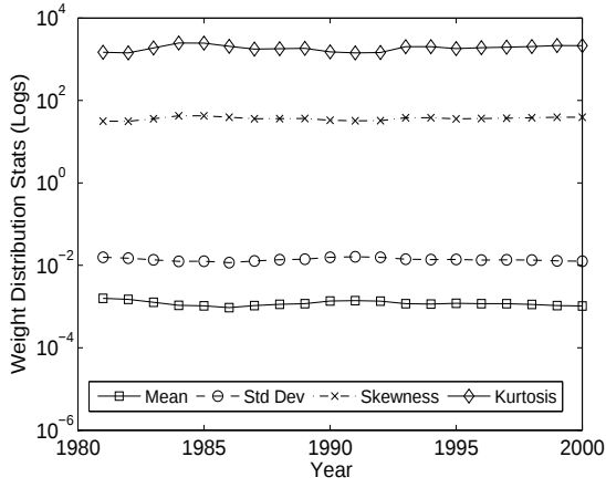
FIG. 1: Sample moments of the link-weight distribution vs. years. Log scale on Y-axis.
