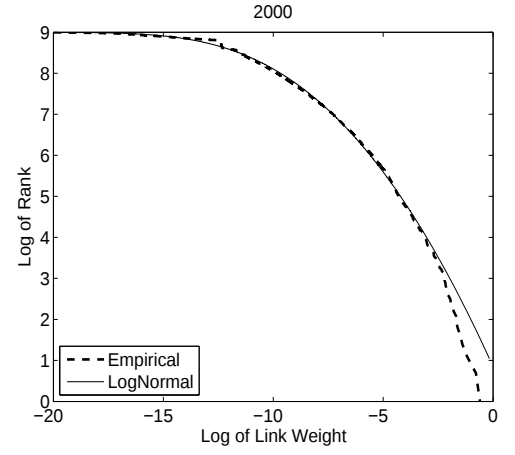
FIG. 2: Size-rank (log-log) plot of the link-weight distribution in year 2000.
