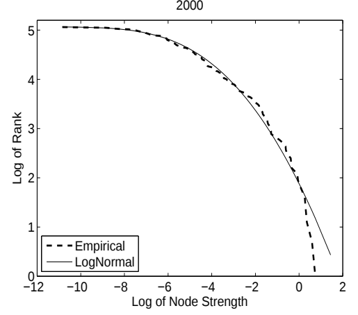
FIG. 5: Size-rank (log-log) plot of node-strength distribution in year 2000.
