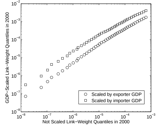
FIG. 19: Quantile-quantile plots of logged link-weight distributions in year 2000. X-axis: Quantiles of logged link-weight distribution for the baseline weighting scheme. Y-axis: Quantiles of logged link-weight distributions in the two alternative weighting schemes analyzed. First scheme: Exports scaled by exporter GDP. Second scheme: Exports scaled by importer GDP.
