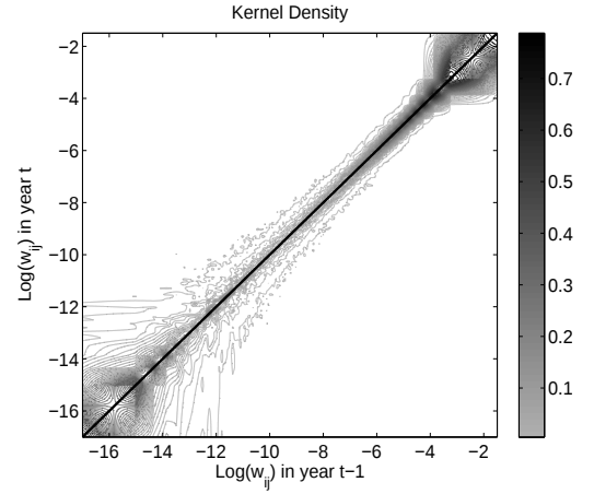
FIG. 13: Contour plot of stochastic-kernel estimates for logged positive link-weights ( \log(w_{ij}^t), w_{ij}^t > 0 ). Solid line: Main 45° diagonal.
