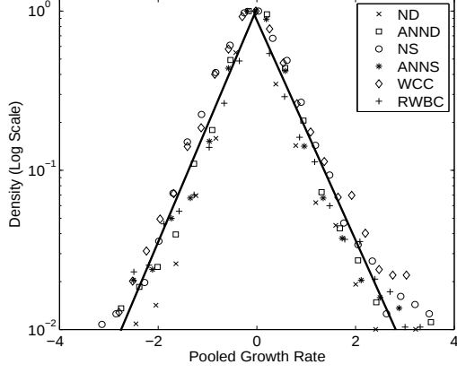
FIG. 14: Pooled growth-rate distributions for node statistics. Y-axis: Log Scale. Solid lines: Laplace fit.
