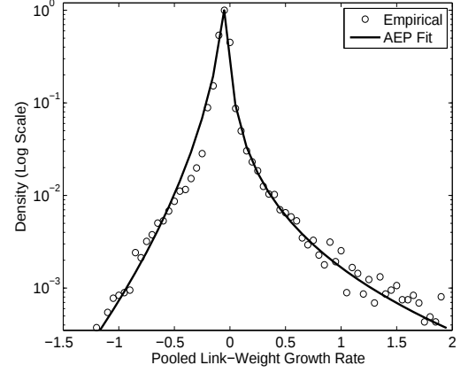
FIG. 15: Pooled growth-rate distribution of link weights. Y-axis: Log Scale. Solid lines: Asymmetric exponential-power (AEP) fit (6). Parameter estimates: \hat{b}_l = 0.5026 , \hat{b}_r = 0.2636 , \hat{a}_l = 0.0511 , \hat{a}_r = 0.0615 , \hat{m} = -0.0202 .
