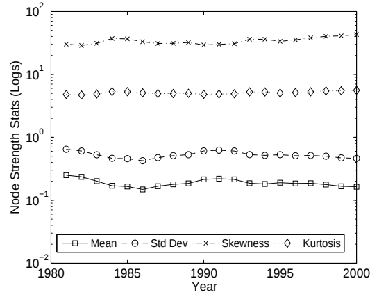
FIG. 3: Sample moments of the node strength (NS) distribution vs. years. Log scale on Y-axis.
