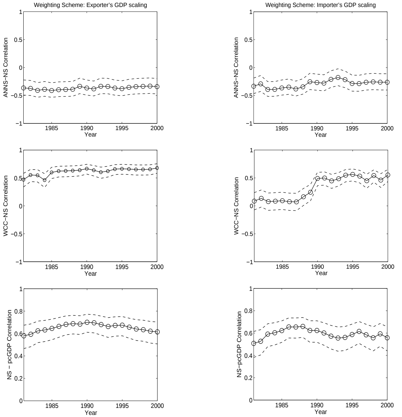
FIG. 20: Correlation structure among node statistics in the two alternative weighting schemes analyzed. Left figures: Exports scaled by exporter GDP. Right Figures: Exports scaled by importer GDP. Dotted lines: 95% confidence intervals for population averages.
