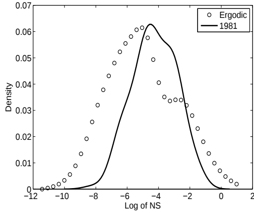
FIG. 16: Node Strength (NS): Kernel density of initial distribution (year=1981) vs. estimate of ergodic (limiting) distribution.
