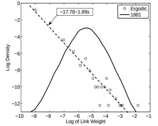
FIG. 17: Positive link weights: Kernel density of initial distribution (year=1981) vs. estimate of ergodic (limiting) distribution. Dotted line: Power-law fit (equation shown in inset). Note: Log scale on y-axis.
