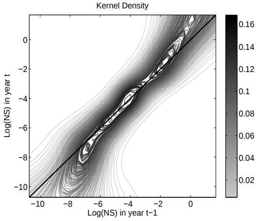
FIG. 12: Contour plot of stochastic-kernel estimates for logged node strength (NS). Solid line: Main 45° diagonal.
