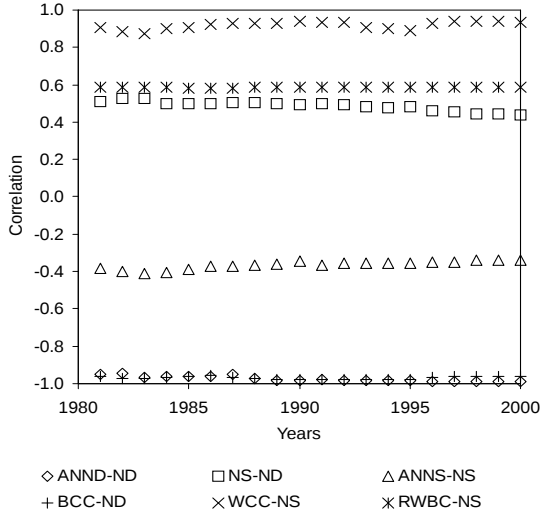
FIG. 10: Correlation between node statistics vs. years.
