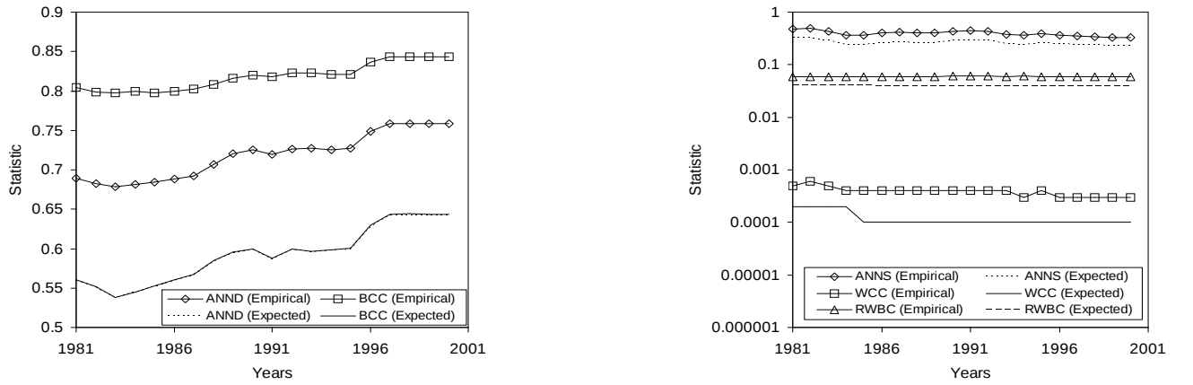
FIG. 9: Population average vs. expected values of node statistics. Expected values for binary-network statistics (left) are computed by reshuffling binary links by keeping observed density fixed. Expected values for weighted-network statistics (right) are computed by reshuffling observed link weights while keeping the binary structure fixed.
