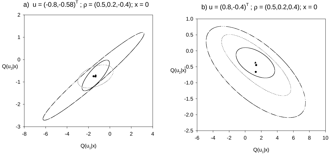
Figure 1: 95% confidence ellipses for Q(u|x) for n = 100 (dash-dotted-dotted lines), n = 200 (dotted lines), and n = 500 (solid lines); the centers of the ellipses at (\hat{Q}_n(u_1|x), \hat{Q}_n(u_2|x)) are denoted by black dots ( n = 100 ), black squares ( n = 200 ), and black triangles ( n = 500 ).
