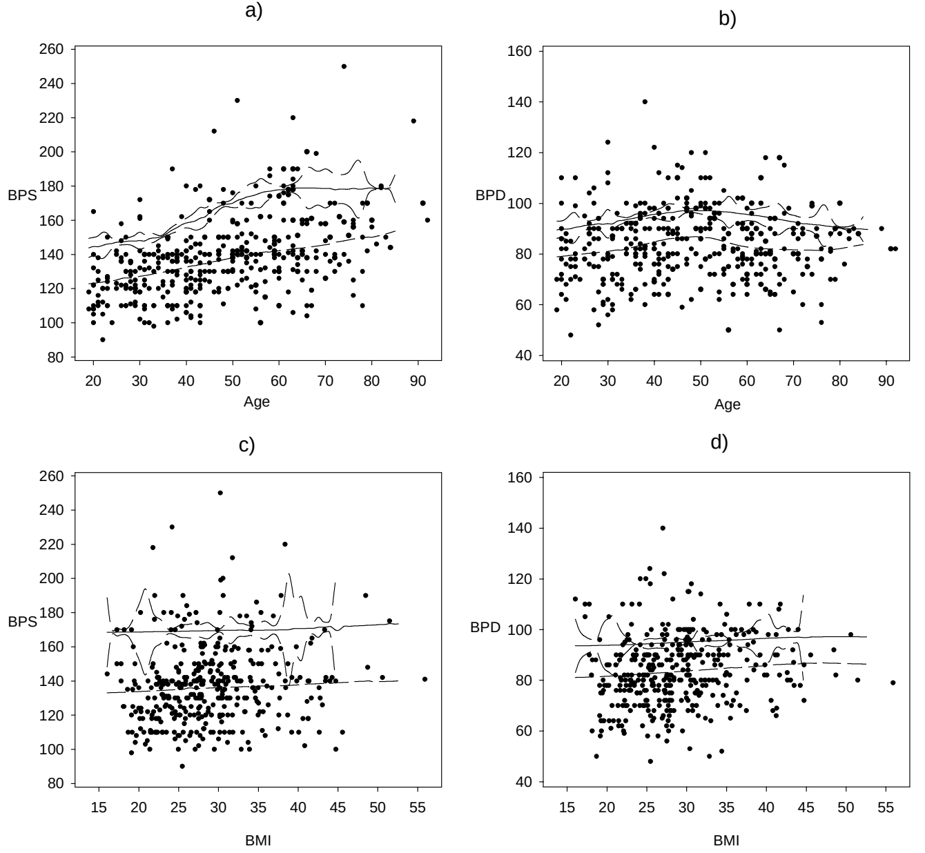
Figure 3: Scatter-plots of BPS and BPD versus Age and BMI . Median-dashed lines are conditional median curves; solid lines are \hat{Q}_n(u|x) 's with u = (0.8, 0.58)^T and long-dashed lines are the associated asymptotic 95% confidence bands.
