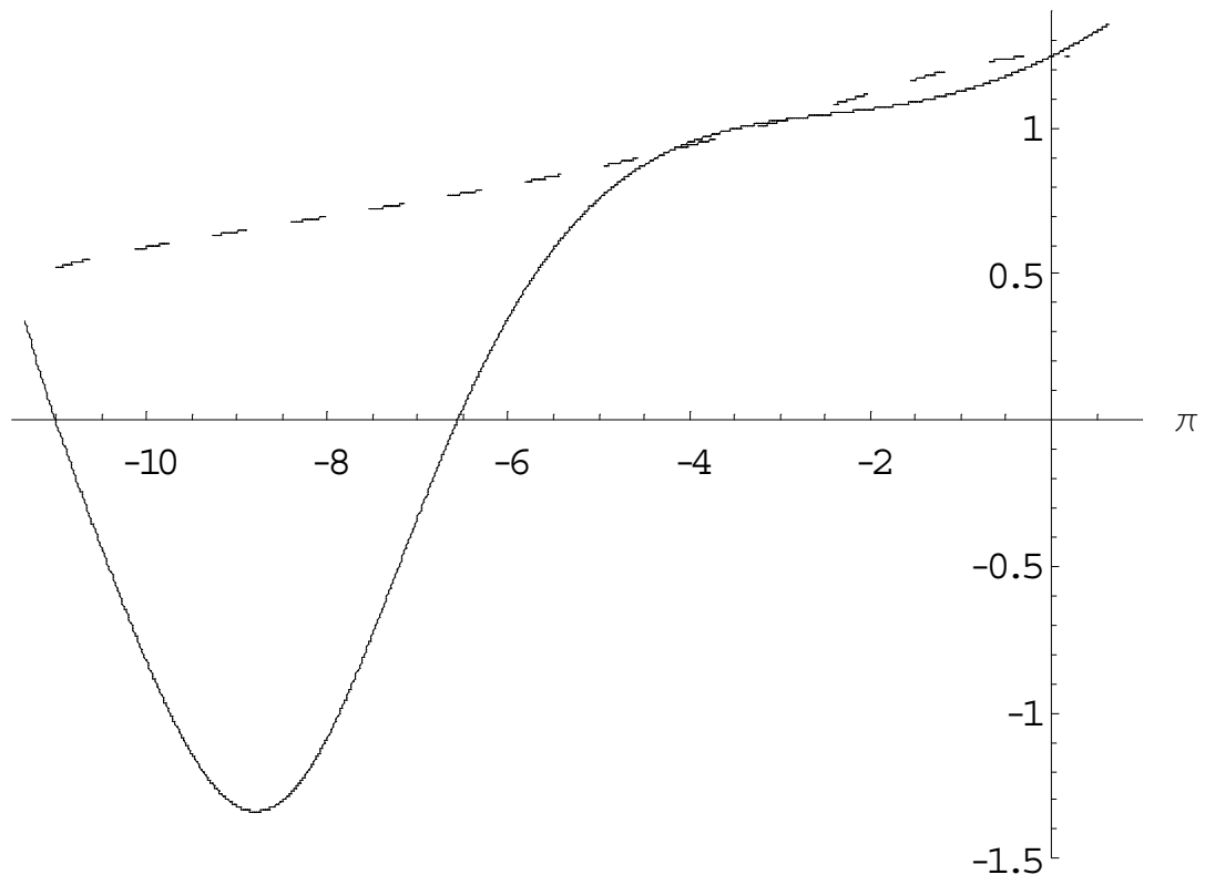
Figure 2: -T \times \text{bias} in the AD(1,0) model for (\pi, \gamma) along Line 1 in Figure 1. Solid line refers to the correct bias approximation -T B'_\lambda(T^{-1}) and the dashed line refers to the incorrect bias approximation -T B_\lambda^{GS}(T^{-1}) .
