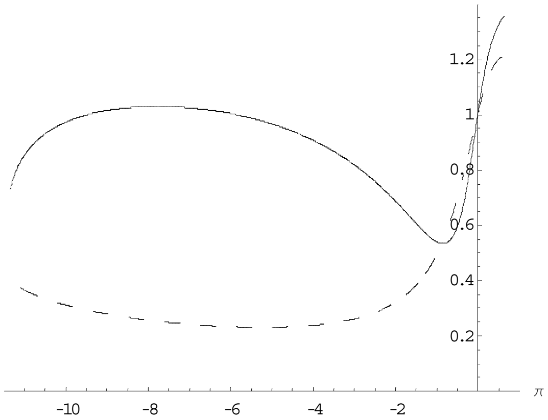
Figure 3: -T \times \text{bias} in the AD(1,0) model for (\pi, \gamma) along Line 2 in Figure 1. Solid line refers to the correct bias approximation -T B_{\lambda}^r(T^{-1}) and the dashed line refers to the incorrect bias approximation -T B_{\lambda}^{GS}(T^{-1}) .
