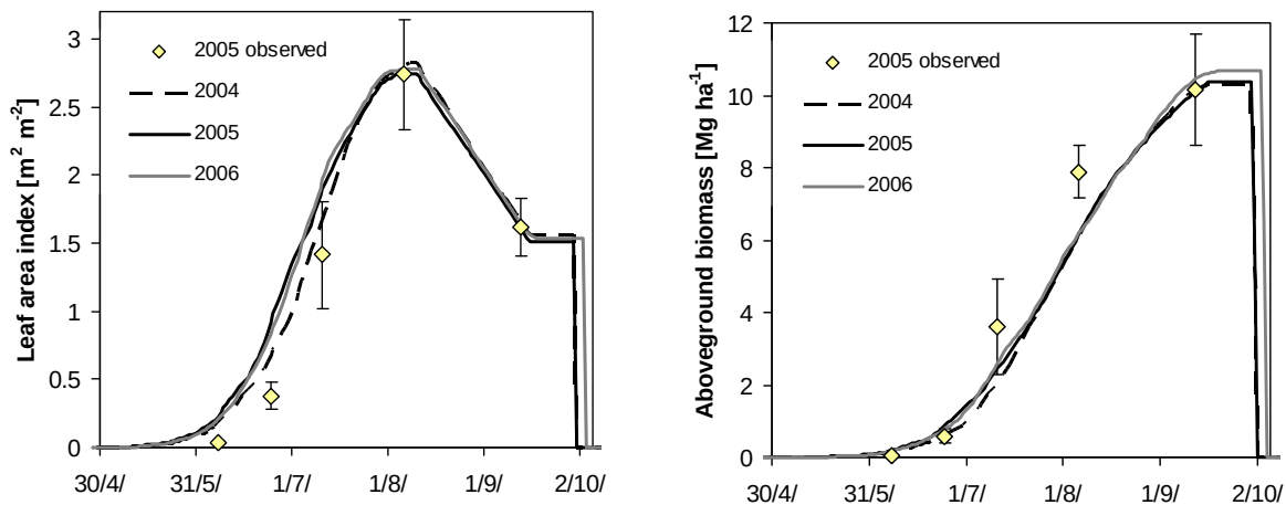
Figure 24: Observed (points) and simulated (lines) leaf area index (left) and aboveground biomass (right) in 2005, as well as simulated LAI and AGB in 2004 and 2006; bars denote the standard deviation
