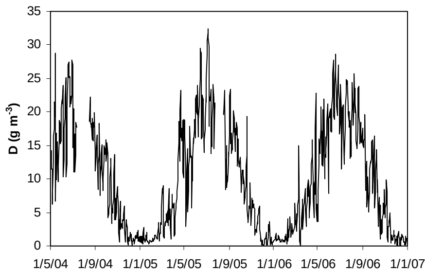
Figure 4: Vapor pressure deficit, D \text{ (g m}^{-3}\text{)} , from 1 May 2004 till end of 2006 at station "Maxhud garden" ( 41^{\circ}36'10.92'' N 60^{\circ}30'50.60'' E, 96 m above sea level)
