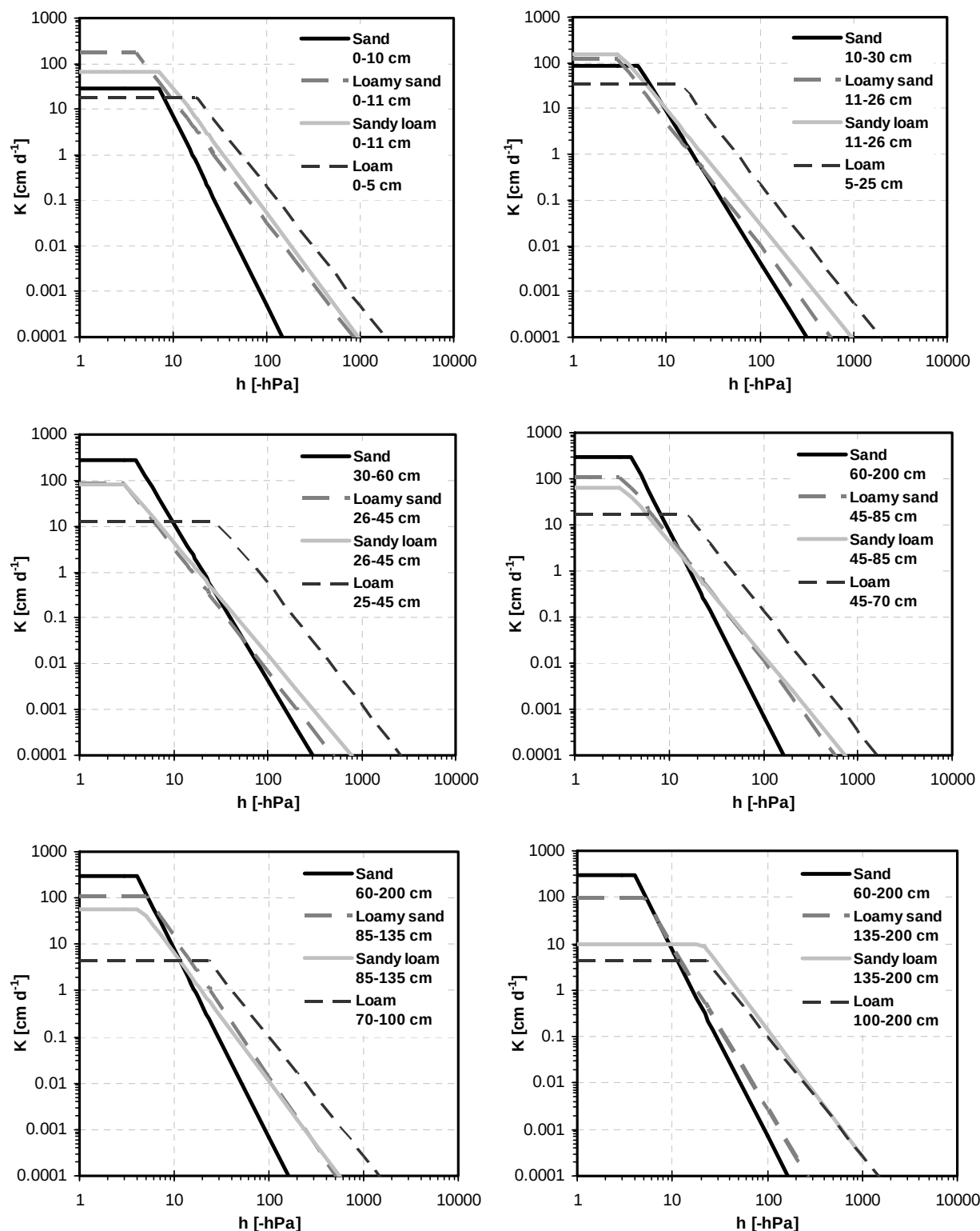
Figure 11: Soil hydraulic conductivity – pressure head, K(h) , curve of the different soil layers of the sand, loamy sand, sandy loam and loam; for easy comparison conductivity of sand at 60–200 cm is shown in three graphs
