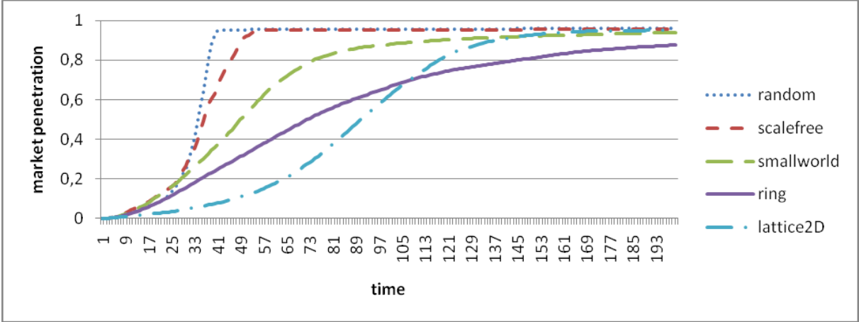
FIGURE 1 Diffusion curves for different network topologies
