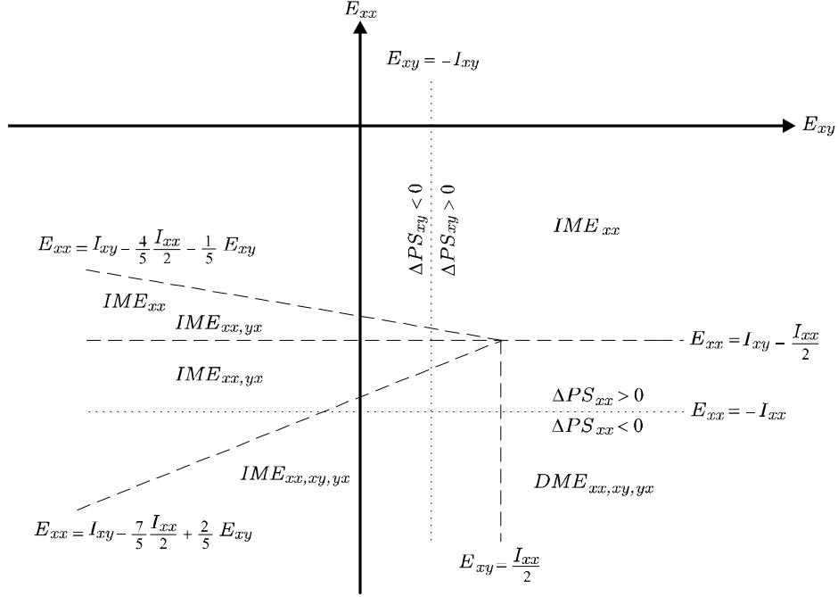
Figure 3: I_{xx} > 0 and \frac{I_{xx}}{2} > I_{xy} .
