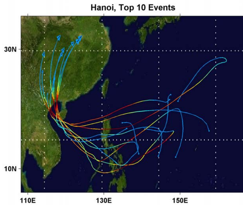
Figure 3: Storm tracks
