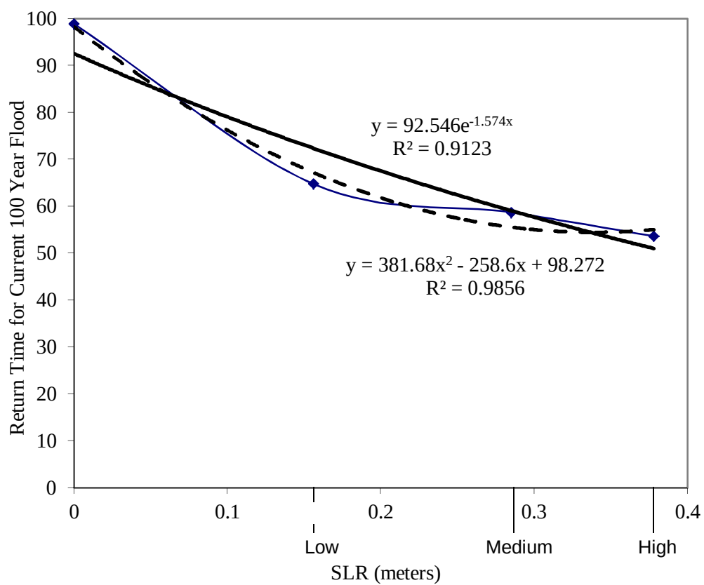
Figure 6: Estimated change in effective return time for the 100-year storm as a result of SLR
