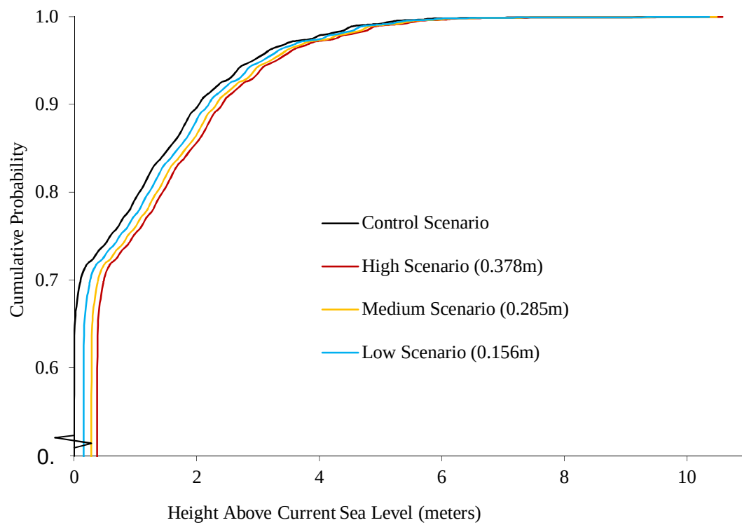
Figure 5: SLOSH-estimated storm surge exceedance curve, with and without SLR
