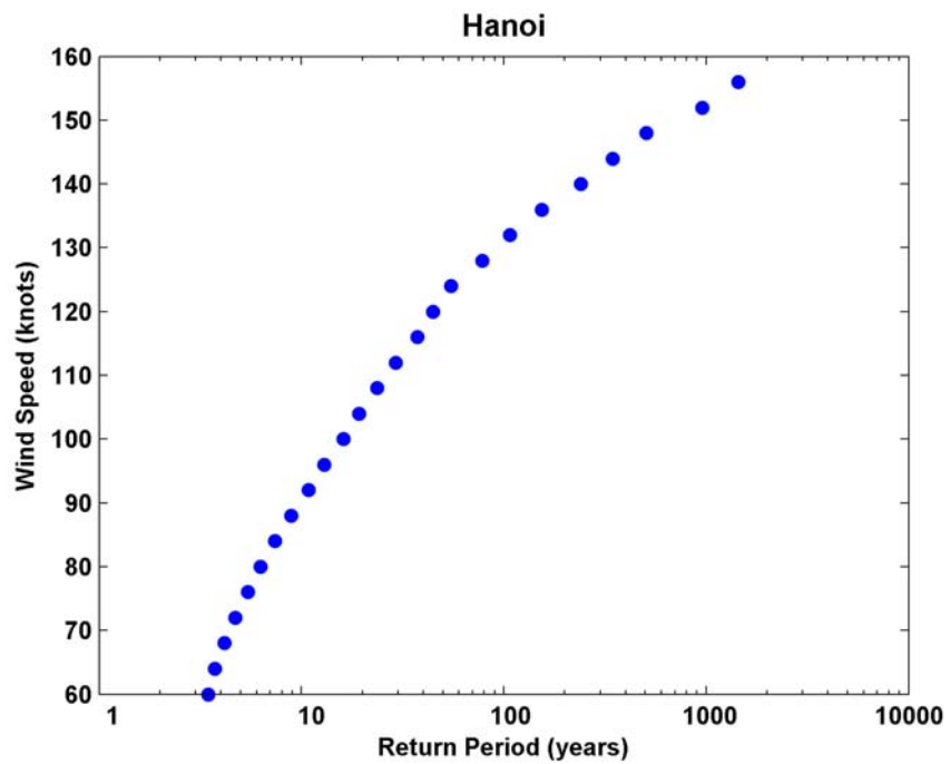
Figure 4: Wind speeds and estimated return times
