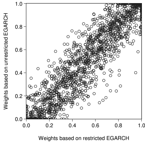
Figure 5: Optimal large firm portfolio weights with and without GARCH spillovers
