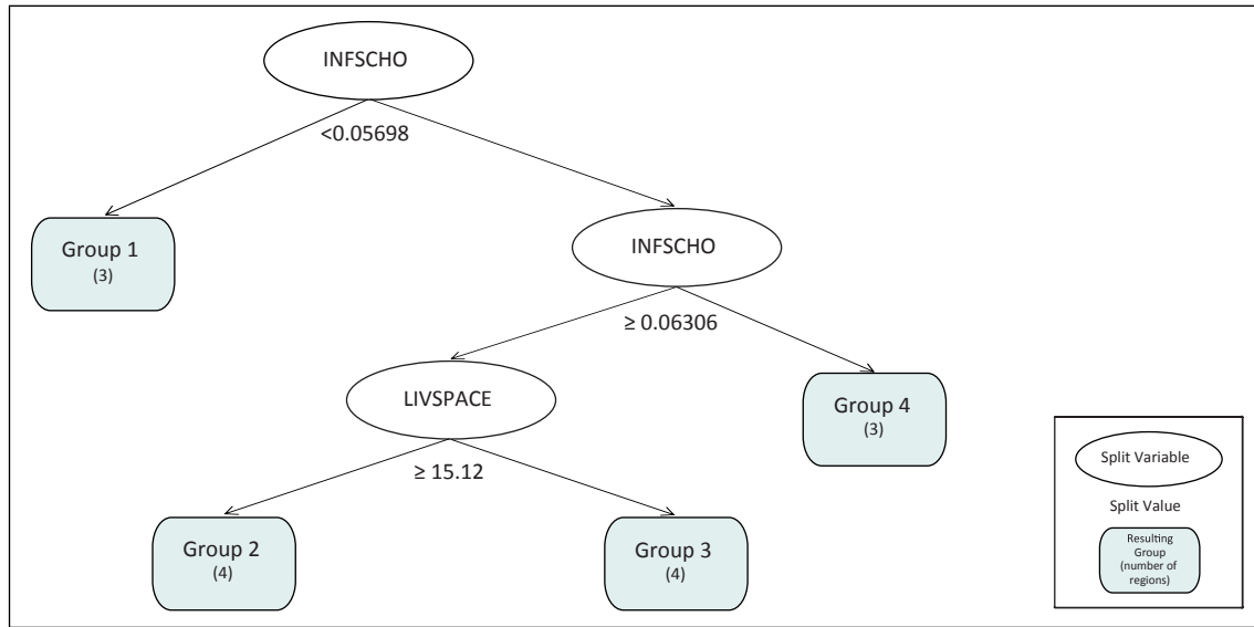
Figure 1: Regression tree
