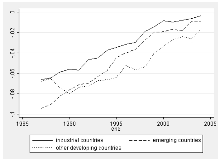
Figure 6: Rolling Regression: Net Foreign Assets
