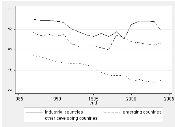
Figure 7: Rolling Regression: net output gap
