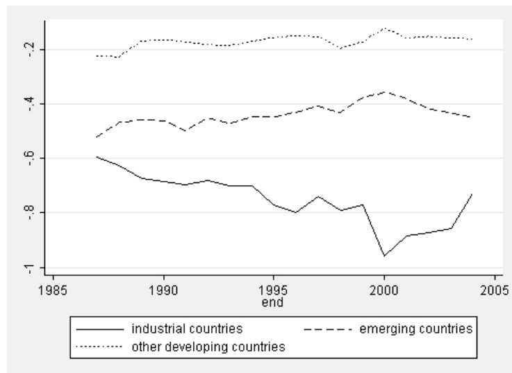
Figure 8: Rolling Regression: lagged net output gap
