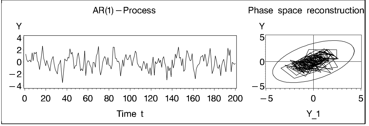
Figure 1: Realization of an AR(1)-process Y_t = 0.5Y_{t-1} + \epsilon_t , \epsilon_t \sim N(0, 1) , t \in \mathbb{N} and its phase space reconstruction; the phase space vectors form an elliptic cloud
