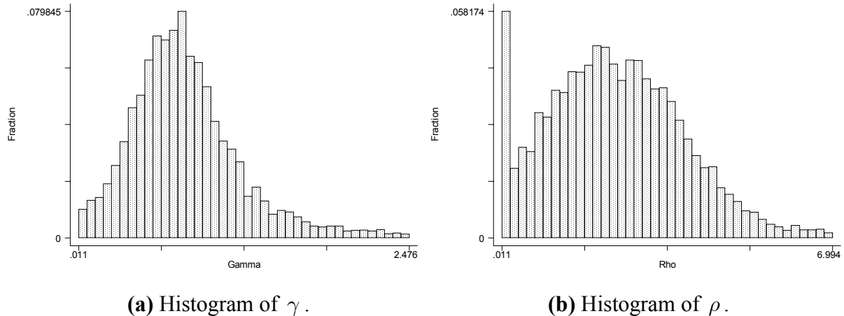
Figure 1. Histogram of Estimated variables.
