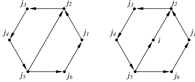
Figure 9: Cycle with diagonal: D_1^D and D_2^D .
