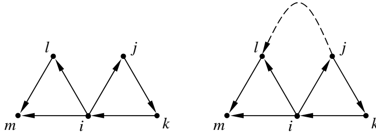
Figure 6: (a) Twin peak network D^{TP} (left), (b) Appended twin peak network D_n^{aTP} (right).
