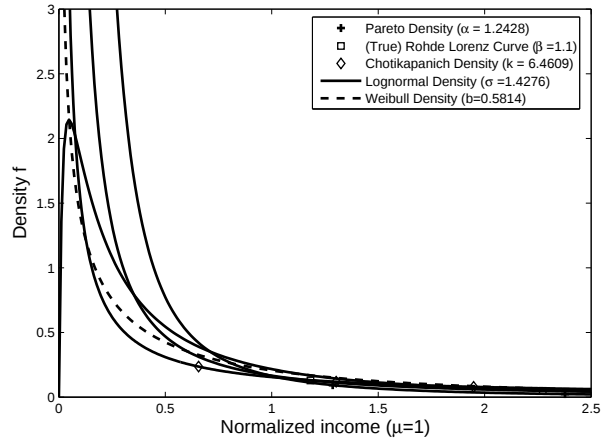
Figure 8: Normalized Densities associated with the LCs from Figure (7)
