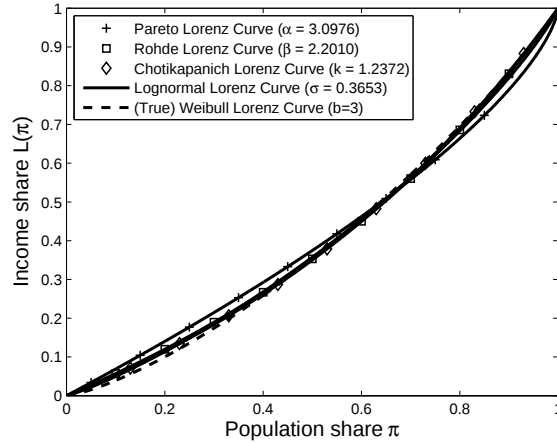
Figure 5: Parametric LCs fitting decile data from a simulated underlying Weibull density ( b = 3 , Gini = 0.2063)
