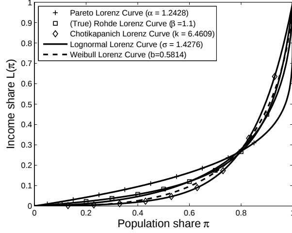
Figure 7: Parametric LCs fitting decile data from a simulated underlying Rohde density ( \beta = 1.1 , Gini = 0.6725)
