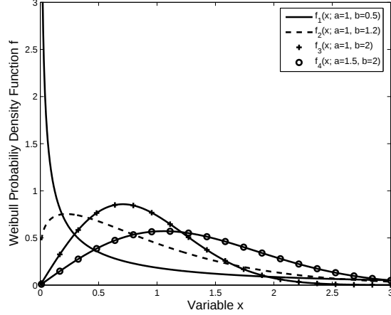
Figure 3: Weibull Density Functions with different a and b parameters
