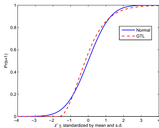
(b) Pr(s_i = 1) : GTL versus Probit
