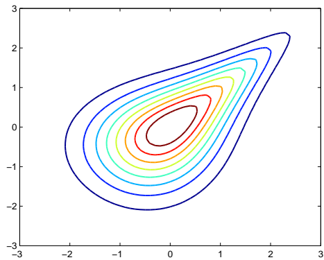
(f) Joe copula: \theta = 1.9050
