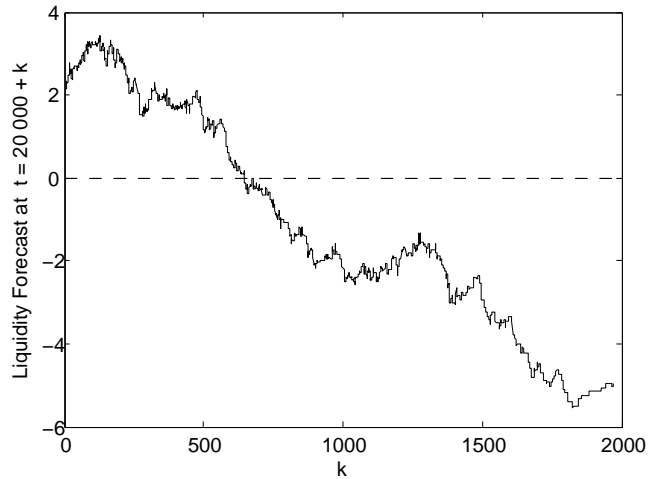
Figure 10: Liquidity Forecast for \bar{b} , t = 20\ 000 \dots 22\ 000
