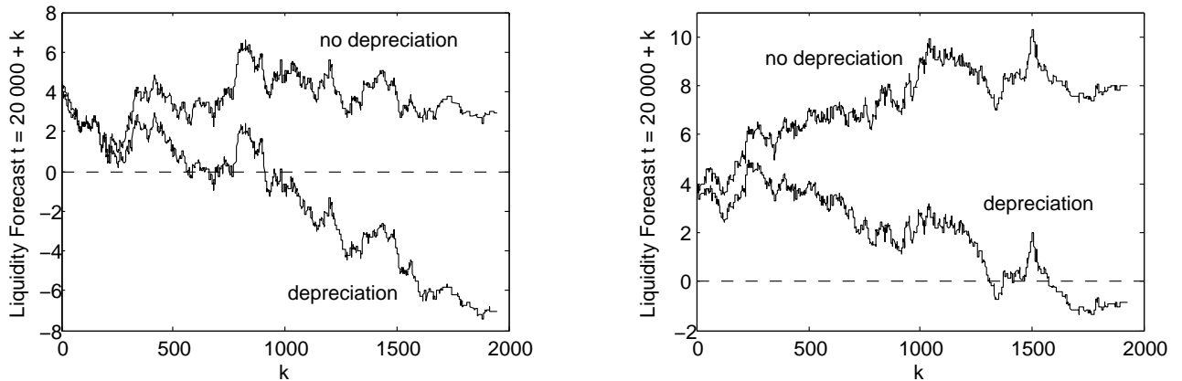
Figure 11: Liquidity Forecasts of two lenders of \bar{b} with and without the depreciation of credits to \bar{b}
