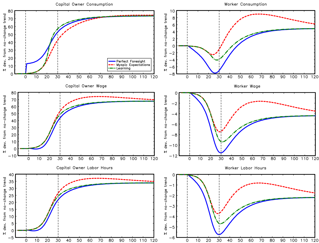
Figure 6: The capital owner’s consumption jumps immediately at t = 1 under perfect foresight. This hinders capital accumulation and lowers the wage trajectories for both capital owners and workers. The myopic expectations regime delivers the most favorable consumption trajectory for workers because faster capital accumulation boosts wages relative to the other two expectation regimes. The transition paths for labor hours mimic the patterns for wages.
