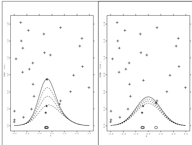
FIGURE 4. X_1, X_2, X_3 vs. Y_1, Y_2, Y_3 .
