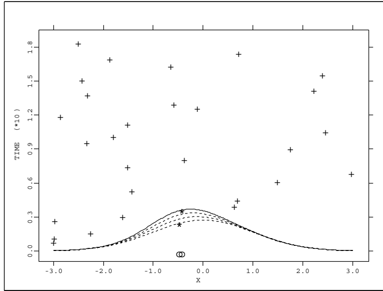
FIGURE 3. Process of determining (U_{j_2}, V_{j_2}) .
