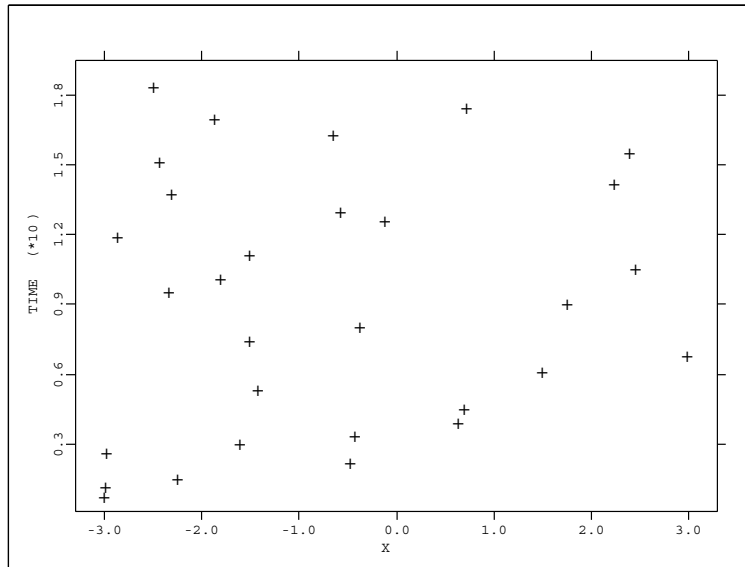
FIGURE 1. Realization of the Poisson process.
