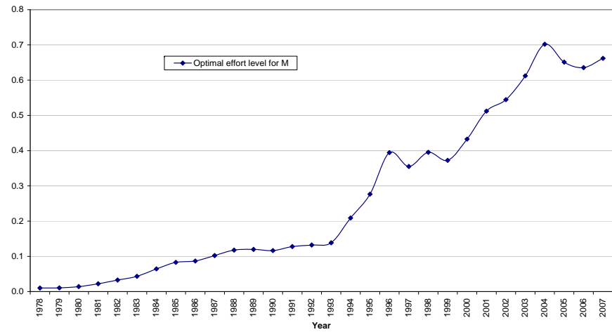
Figure 5b: Optimal effort level for M (Model 3)
