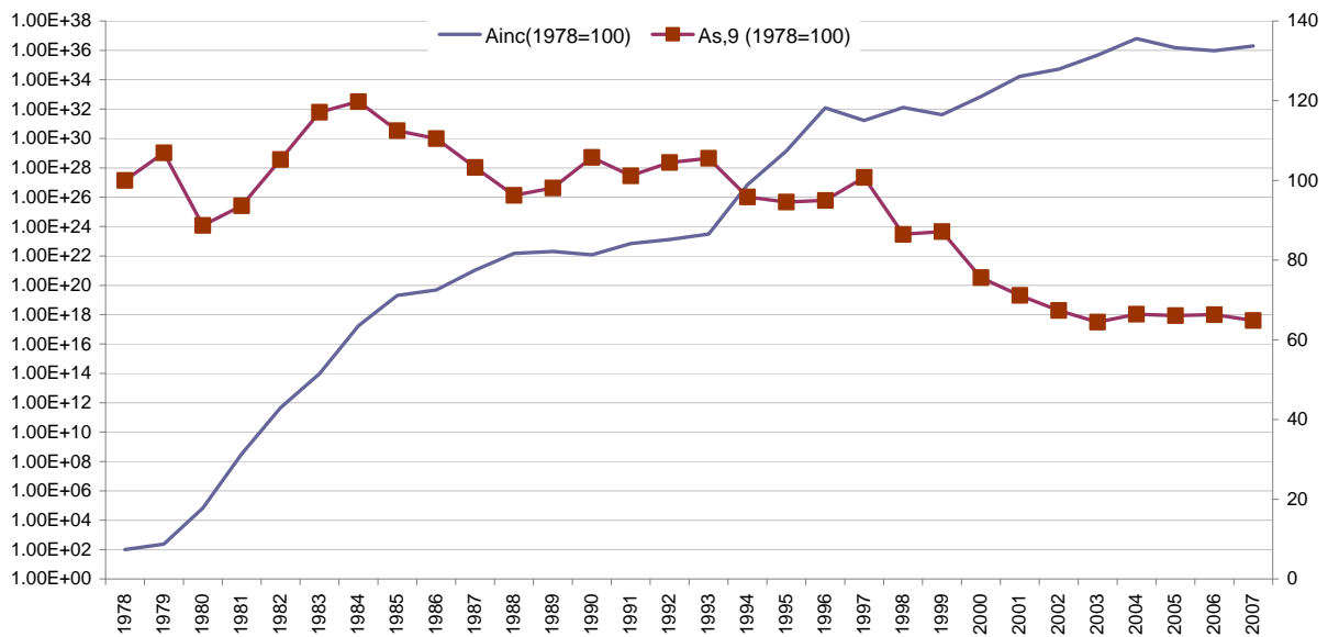
Figure 2b: TFP Index (As) and the index for the incentive component of TFP (Ainc) for Model 9
