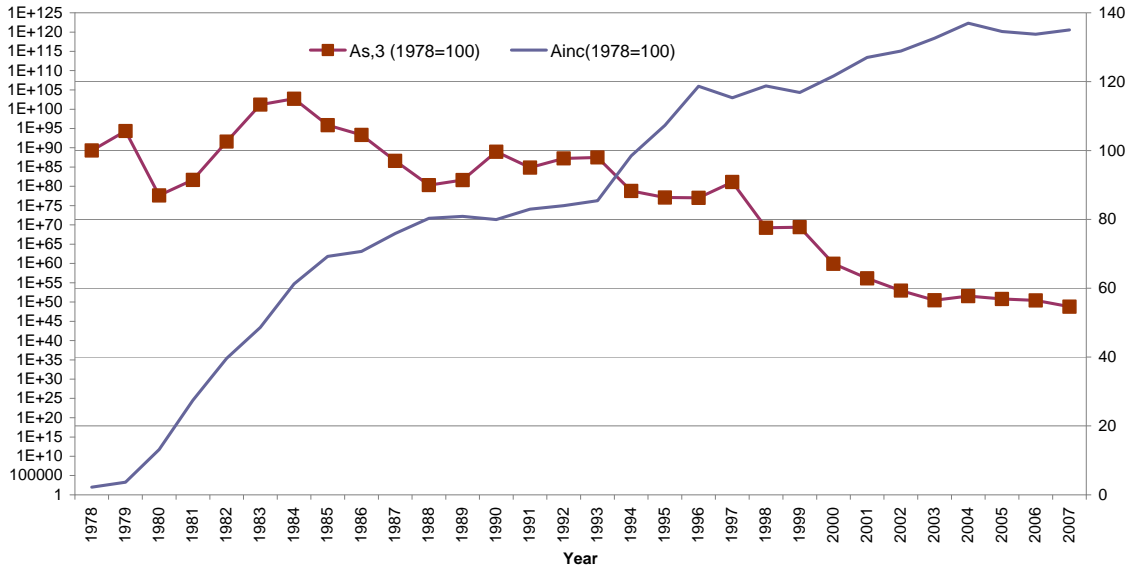
Figure 2a: TFP Index (As) and the index for the incentive component of TFP (Ainc) for Model 3
