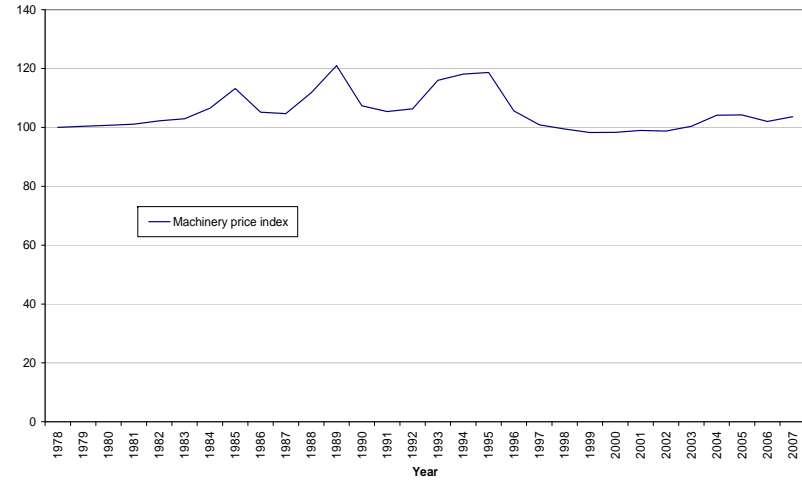
Figure 1b.5: Machinery price index, 1978-2007
