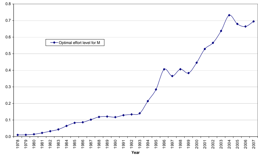
Figure 7b: Optimal effort level for M (Model 9)
