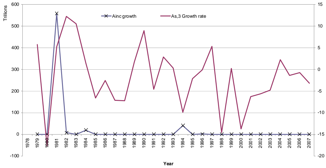
Figure 3a: Growth in TFP (As) and the incentive component of TFP (Ainc) for Model 3
