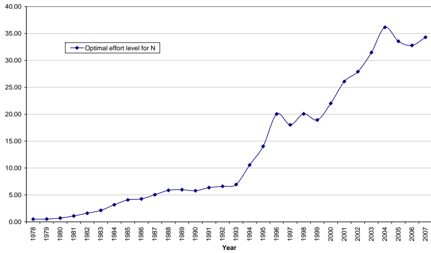
Figure 7a: Optimal effort level for N (Model 9)
