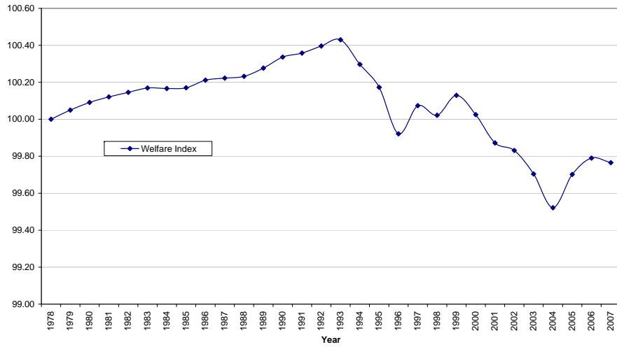
Figure 6a: Welfare Index for Model 9
