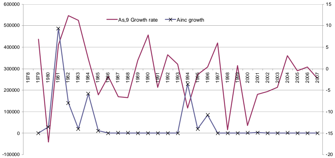
Figure 3b: Growth in TFP (As) and the incentive component of TFP (Ainc) for Model 9
