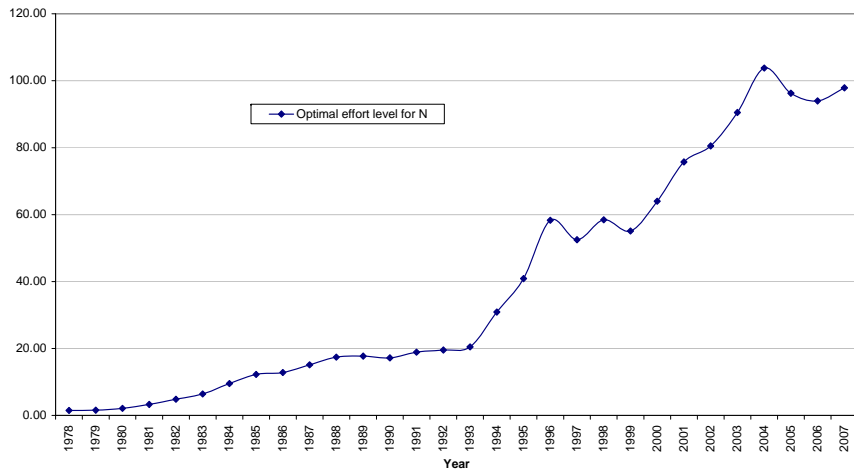
Figure 5a: Optimal effort level for N (Model 3)
