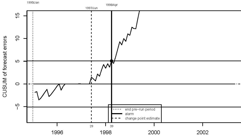
Figure 11: Residual CUSUM chart for the initial model and the first alarm ( k = 0.5 ).
