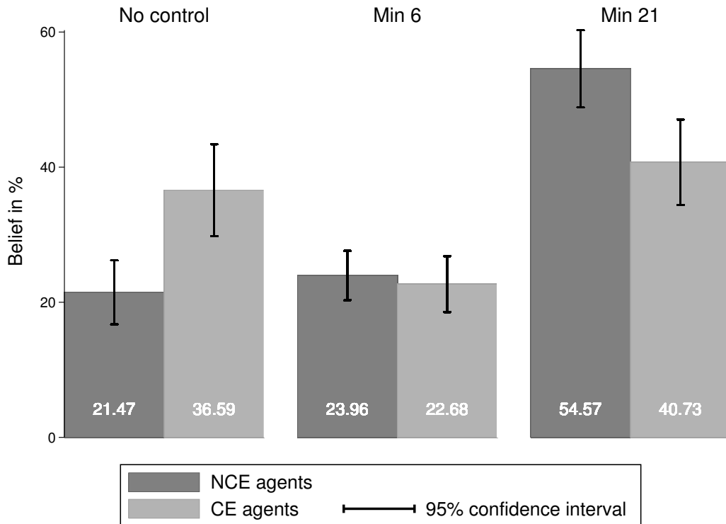
Figure 2: Effort-Choice Game: Agents’ Control Beliefs by Agent Type
