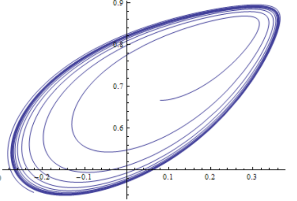
Figure 1b: Initial value q_R = 4.043060432395
