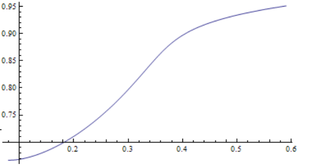
Figure 1d: Initial value q_R = 3.95
