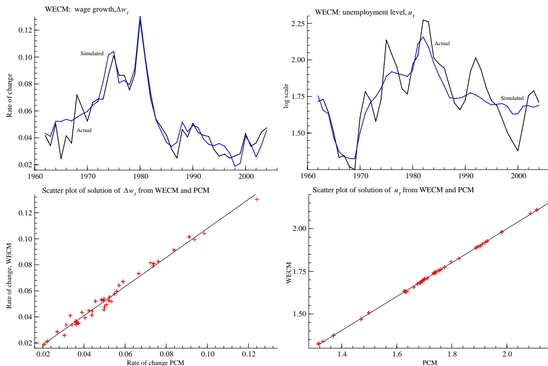
Figure 1: Dynamic simulation of the WECM and PCM. Panel a) shows the WECM solution for \Delta w_t together with the actual value, and panel b) is the same graph for u_t . Panel c) shows the scatter plot of the simulated \Delta w_t values of the WECM and PCM models, with regression line drawn. Panel d) shows the similar graph for the rate of unemployment.
