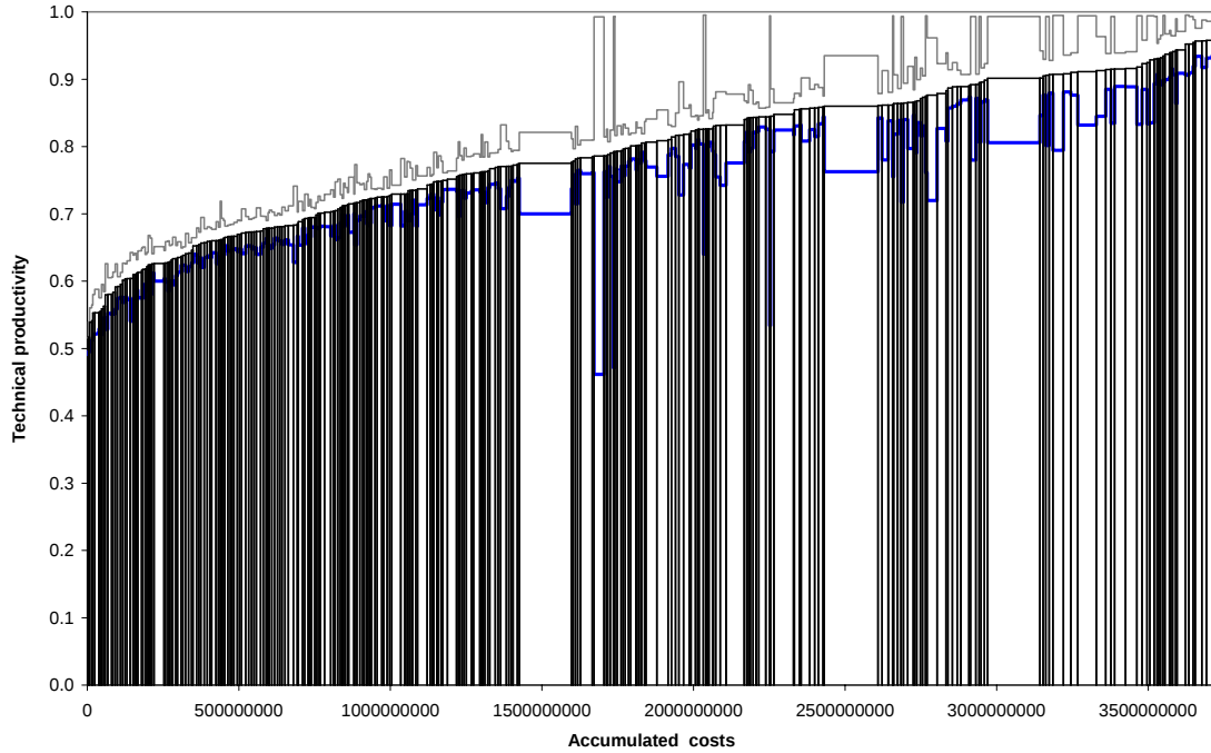
Figure 11. Efficiency relative to optimal scale (technical productivity) 95% confidence intervals
