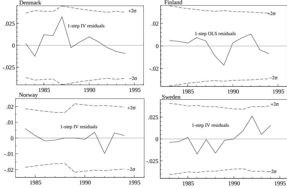
Figure 6: Recursive residuals
