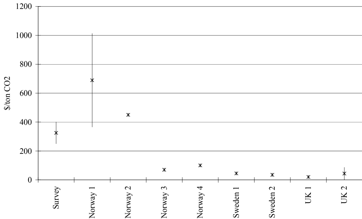
Figure 2. Ancillary benefits of carbon taxes due to reduced air pollution and traffic externalities, per ton reduction in CO 2 emissions.
