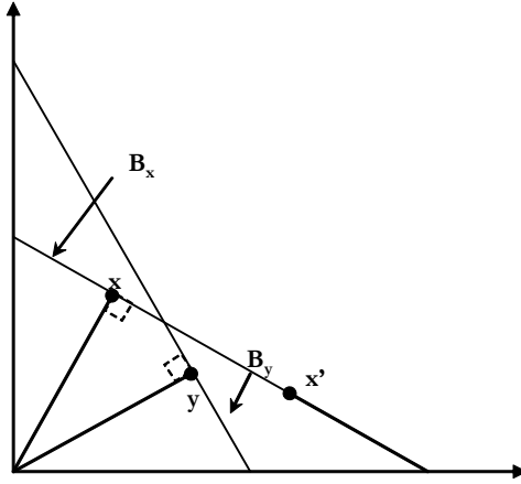
Figure 2: The frugal consumer aggregates with \sum_i z_i^2
