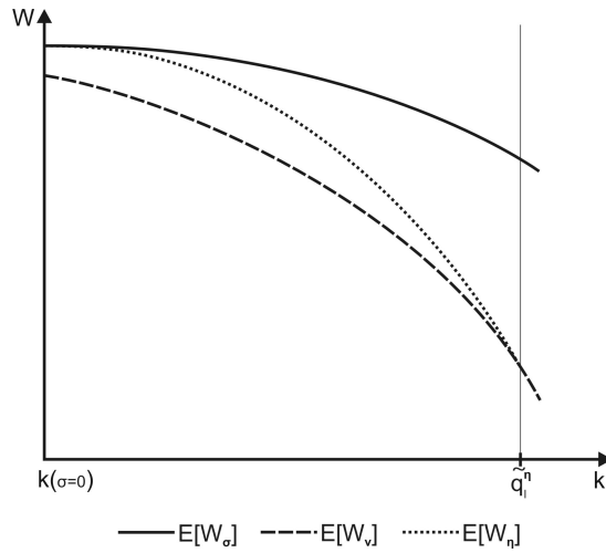
Figure 1: Comparison of promotion schemes in terms of economic surplus.
