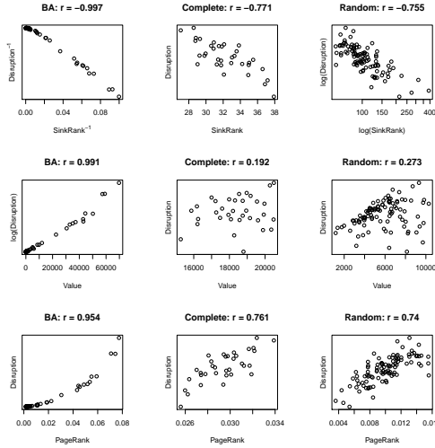
Figure 5: Relationship between disruption and centrality measures in BA, complete, and random networks
