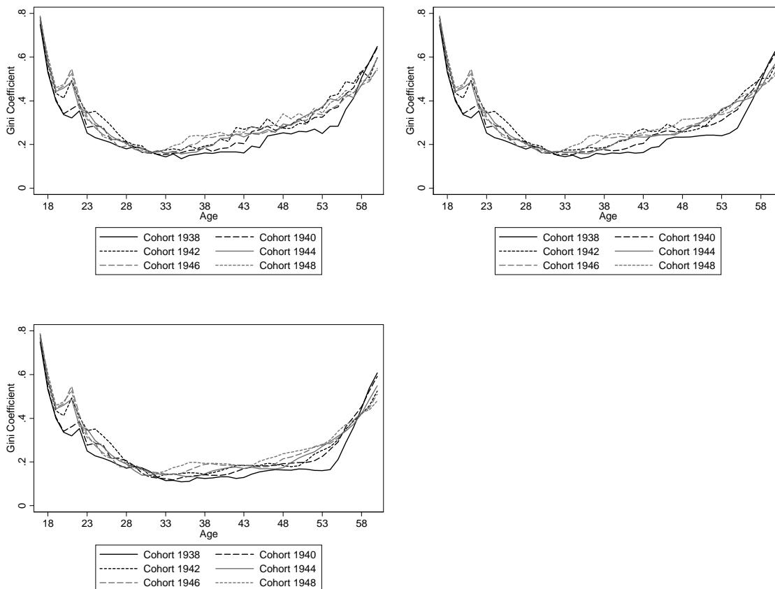
Figure 2 b: Annual Gini coefficients from 17 to 60 for cohorts 1938-1948. Assumption of maximal mobility, mean imputed earning and not imputed earning (in this order).
