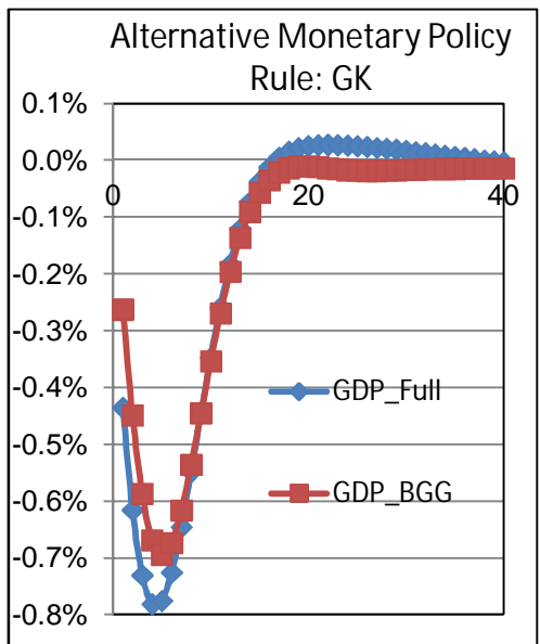
Figure 8a: Technology Shock - Robustness
