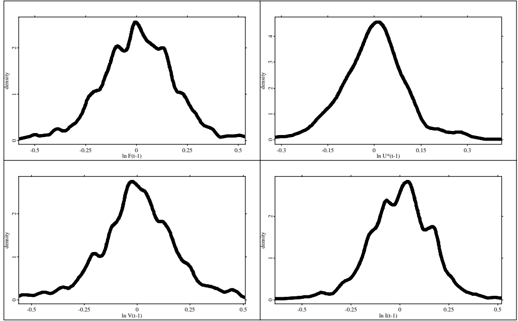
Figure 1c: Density estimates for 1994, upper left: \ln F_{i,t-1} , upper right: \ln U^*_{i,t-1} , lower left: \ln V_{i,t-1} , lower right: \ln I_{i,t-1}
