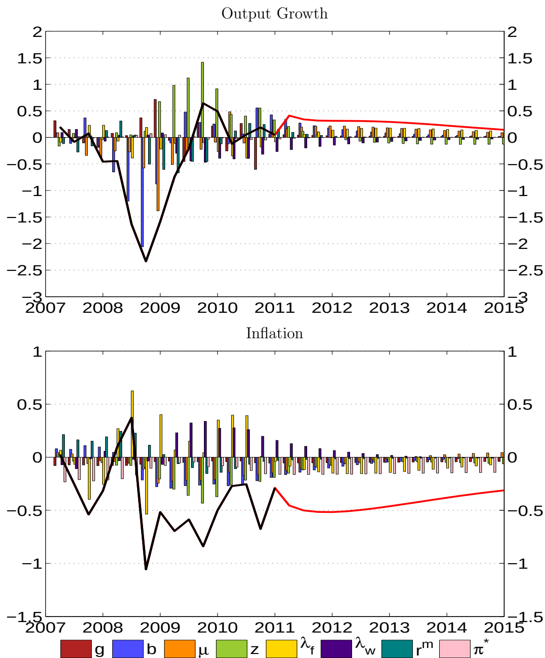
Figure 11: Shock Decompositions
