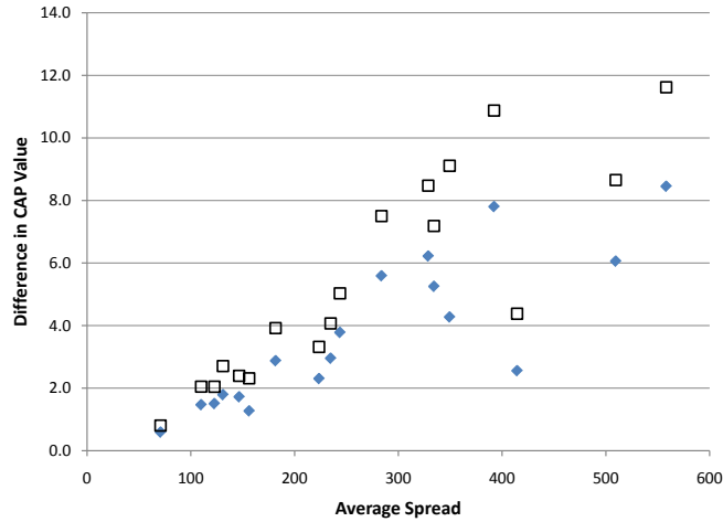
Figure 4: The figure shows differences in CAP values (with and without default) plotted against average CDS spreads. The diamonds mark differences with fixed interest rates, and the squares mark differences with stochastic rates. The correlations are 0.85 and 0.88, respectively.
