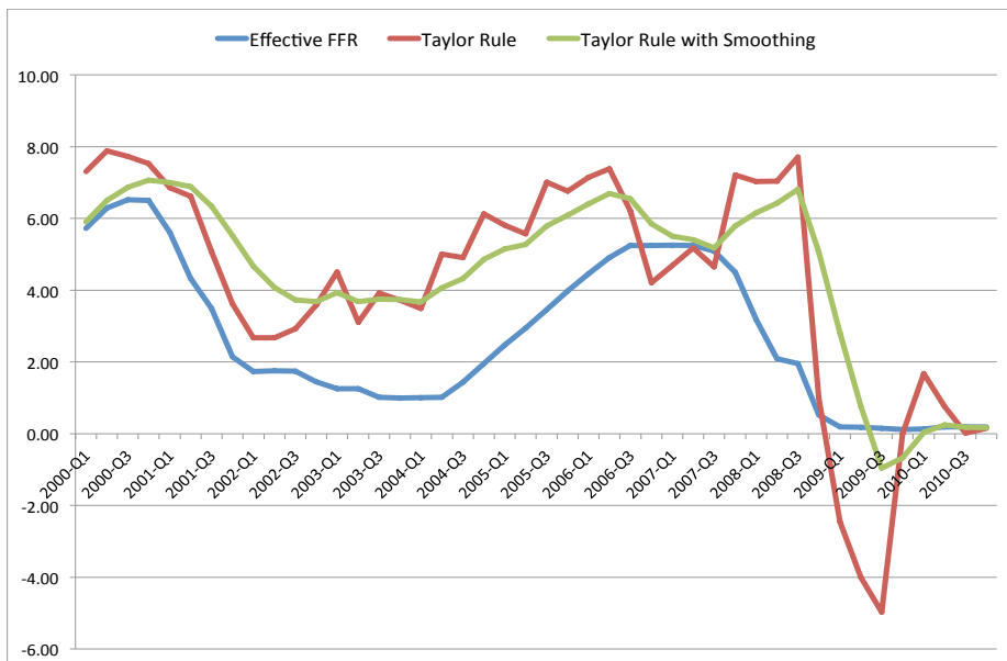
Figure 5: Effective Federal Funds Rate (blue line) and nominal interest rate predicted by a Taylor rule with (green line) and without (red line) smoothing.
