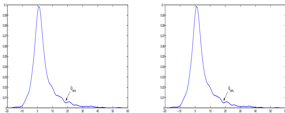
Figure 6: Test distribution for the output gap persistence: GI (left) and GM (right)
