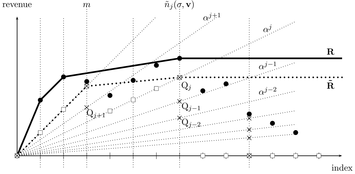
Figure 2: The dotted vertical lines are \lceil c^{d+\sigma} \rceil for d \in \mathbb{Z} ; while the diagonal lines from the origin represent value \alpha^j (as their slopes) for j \in \mathbb{Z} . Each value v_i is represented with “•” at point (i, iv_i) . The line upper-bounding the black dots represents the original revenue curve, \mathbf{R} . For each diagonal line representing \alpha^j , n_j(\mathbf{v}) is the number of values that lie above it; the dotted vertical line immediately to the left of the right-most among these values represents \tilde{n}_j(\sigma, \mathbf{v}) ; finally the intersection between this line and \alpha^j is the point Q_j , represented with “×”. \mathbf{R} and \tilde{\mathbf{v}} are constructed from estimates \tilde{n}_j(\sigma, \mathbf{v}) \geq m and their corresponding Q_j s. The thick dotted function upper-bounding these Q_j s is \tilde{\mathbf{R}} , and each \tilde{v}_i is represented by the point (i, i\tilde{v}_i) with a “□”.
